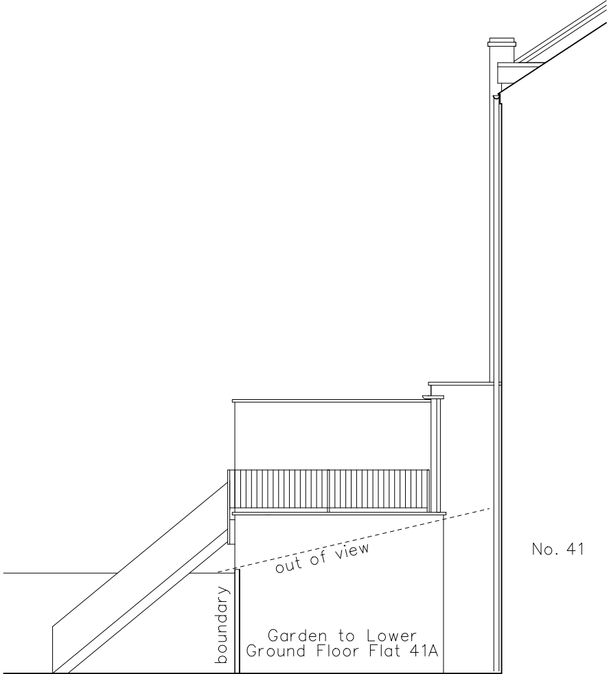
3. SOUTH ELEVATION (Section C through No. 41)
