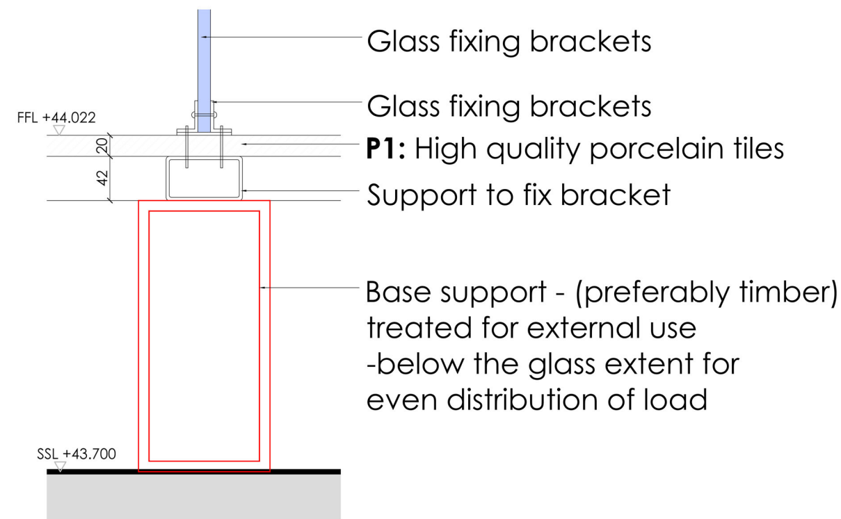
D-07-402 Green House Design Intent - Glass fin fixing detail @ 1:5 03 Hatton Garden
