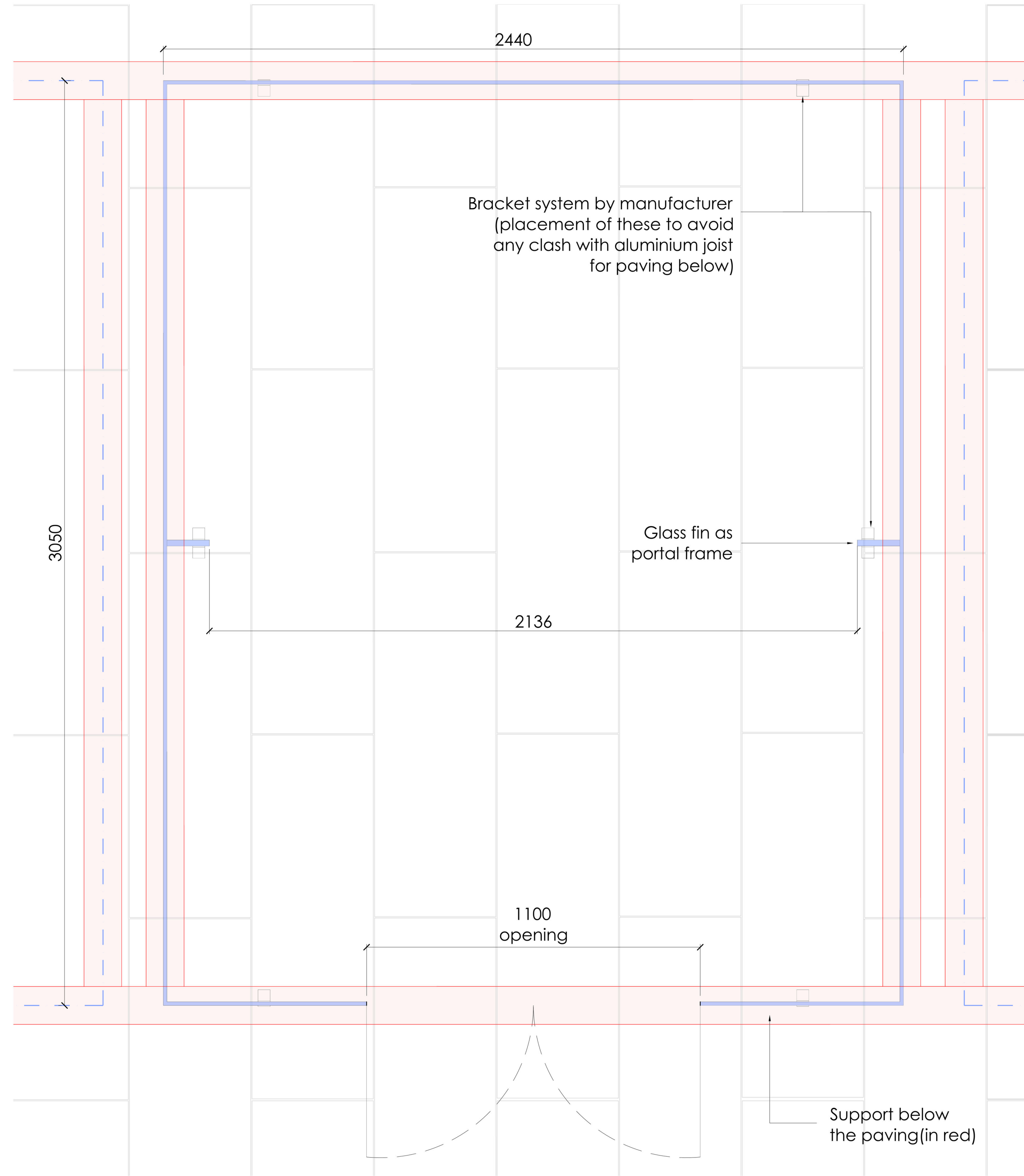
D-07-402 Green House - Plan @ 1:10 01 Hatton Garden
