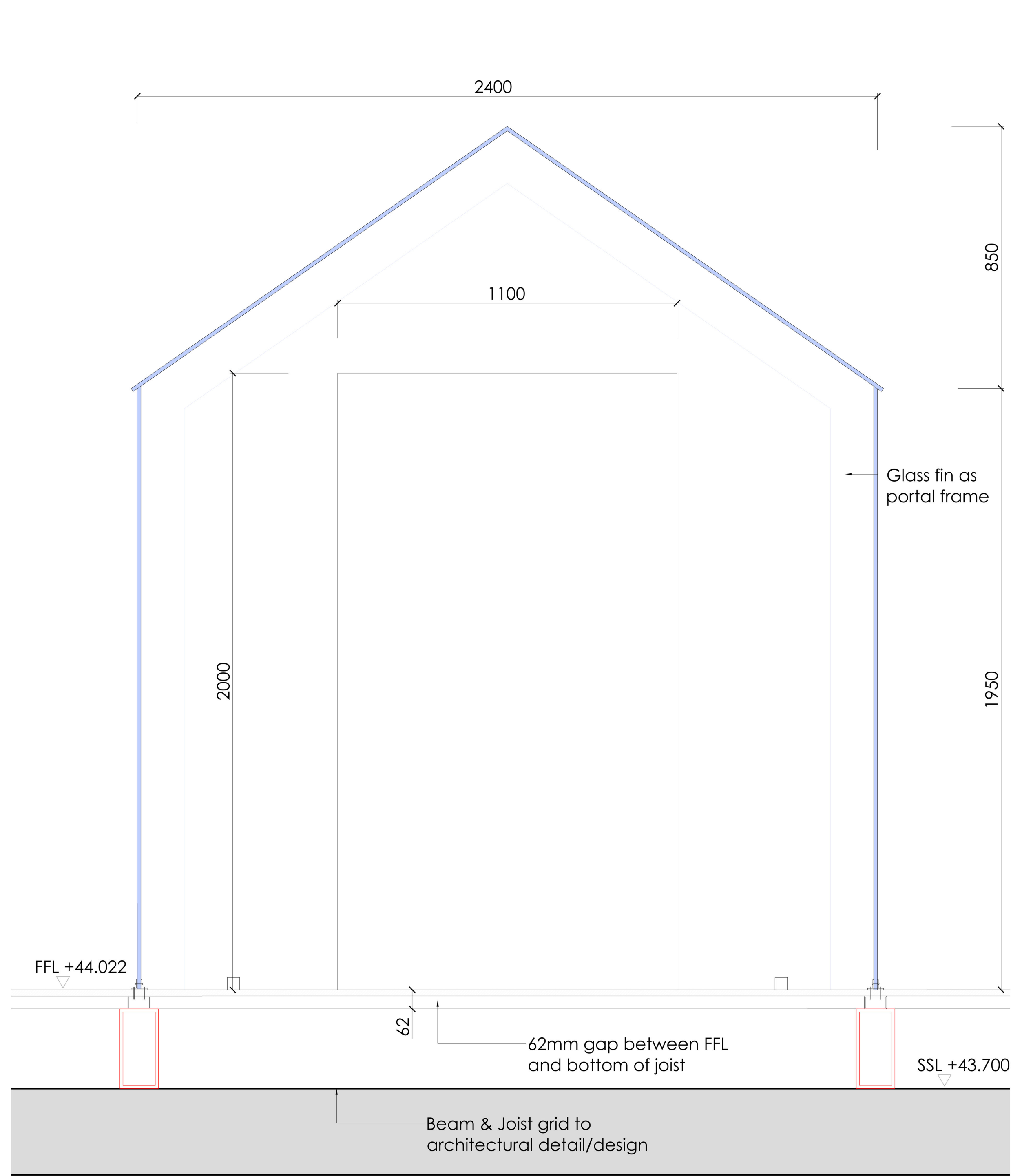
D-07-402 Green House - Section @ 1:10 02 Hatton Garden
