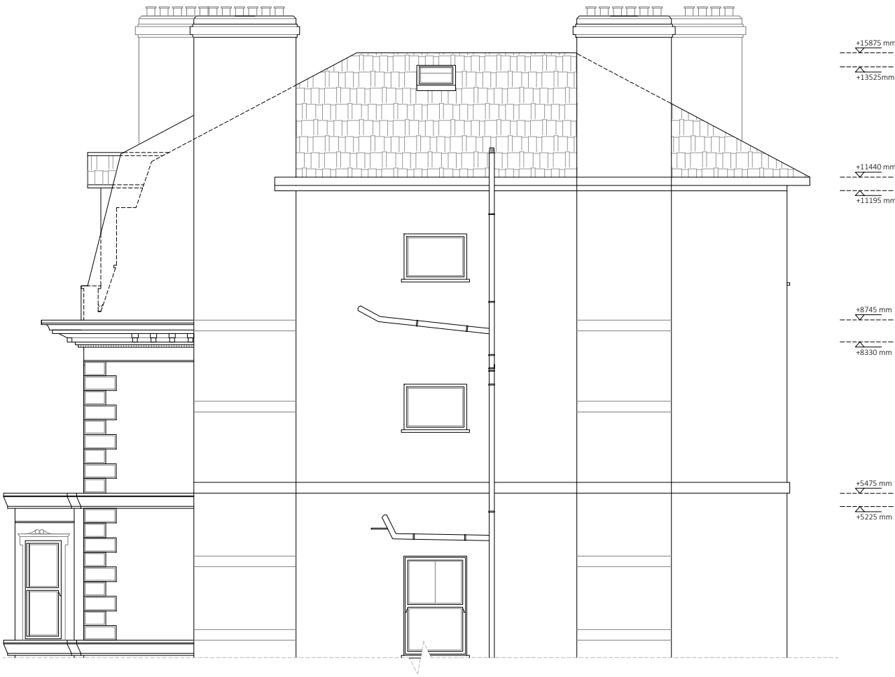
EXISTING EAST SIDE ELEVATION
