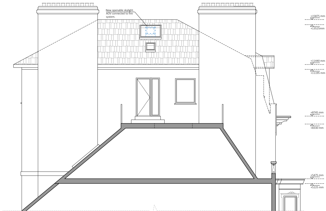
PROPOSED WEST SIDE ELEVATION
