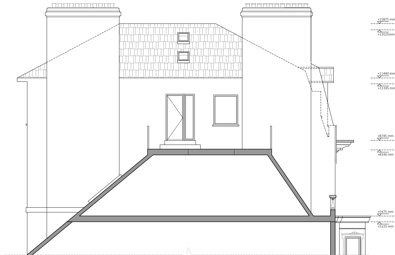
EXISTING WEST SIDE ELEVATION
