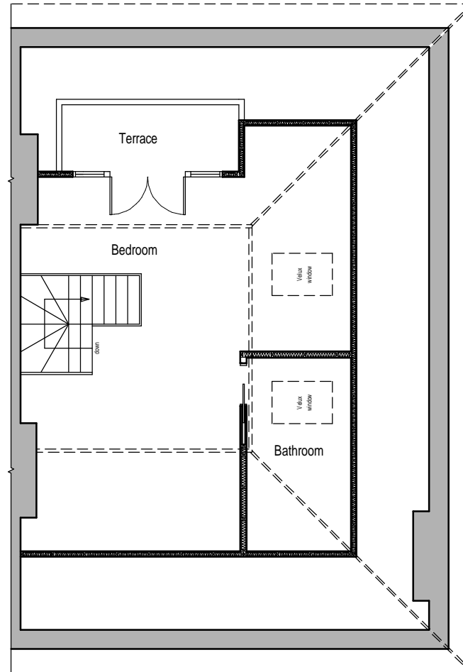
Proposed upper floor plan
