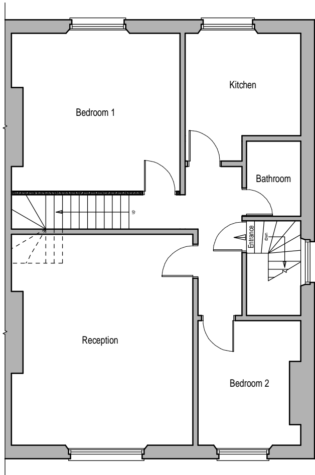
Proposed main floor plan
