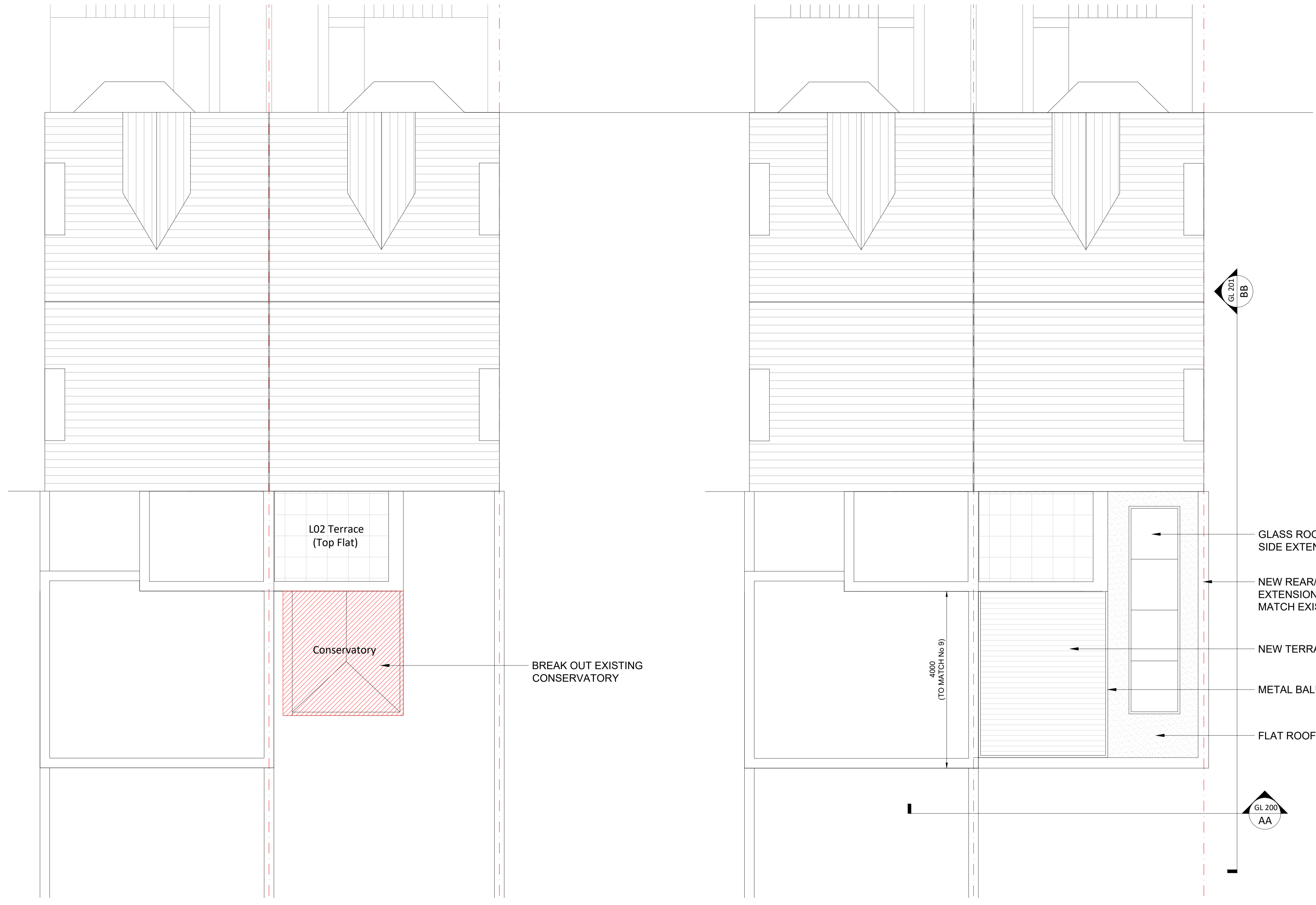
xP Roof EXISTING ROOF PLAN 0 0.5 1 2 3 1:50 at A1
