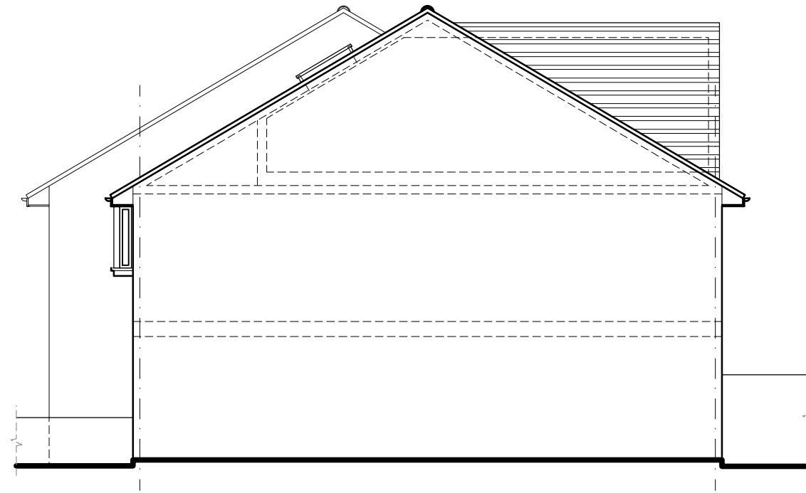
Side Elevation 01
