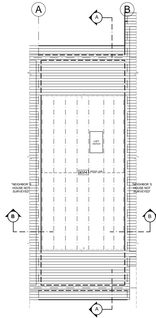
Loft Floor Plan
