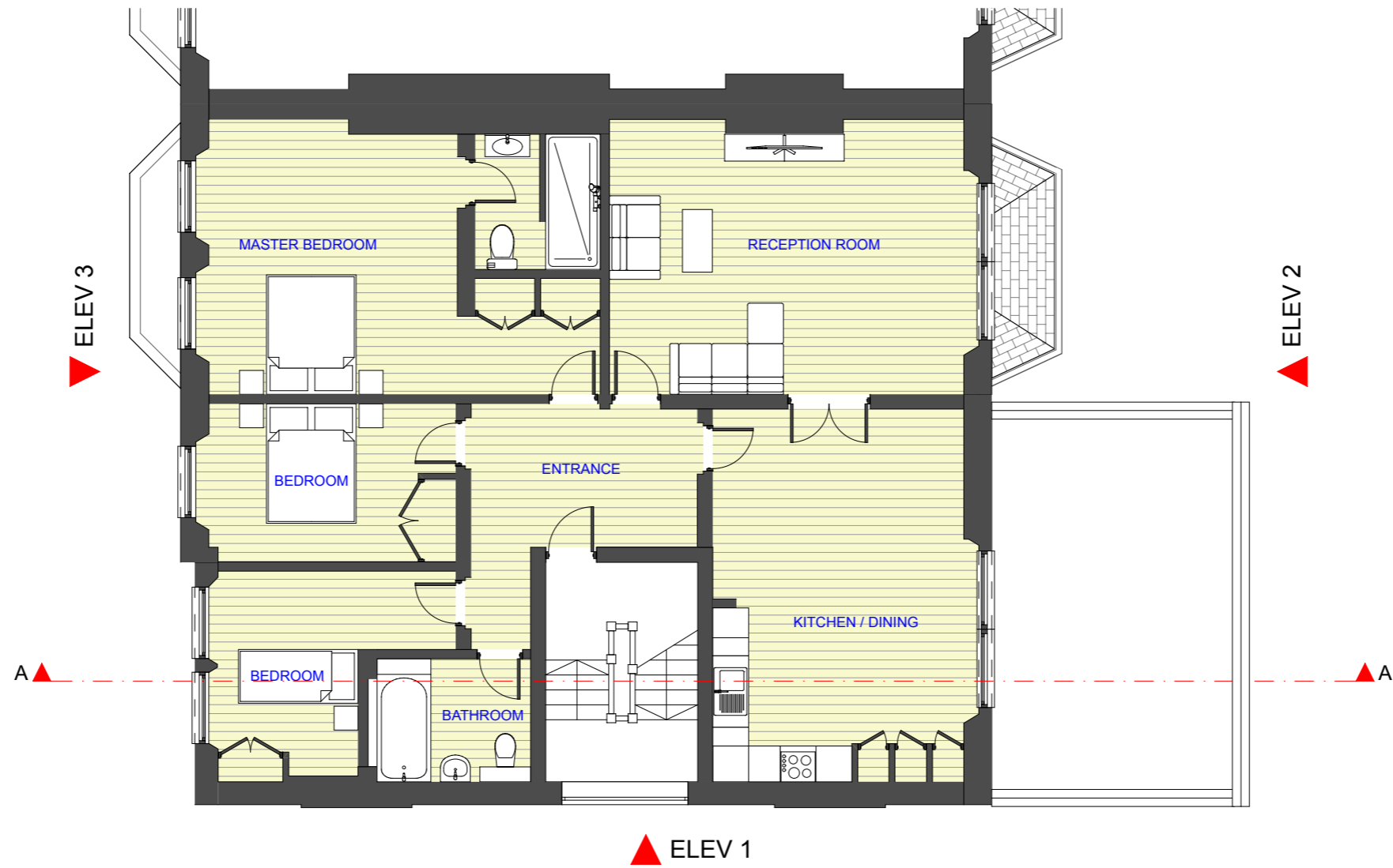
EXISTING FIRST FLOOR PLAN No.12 SCALE @ A3_1:100
