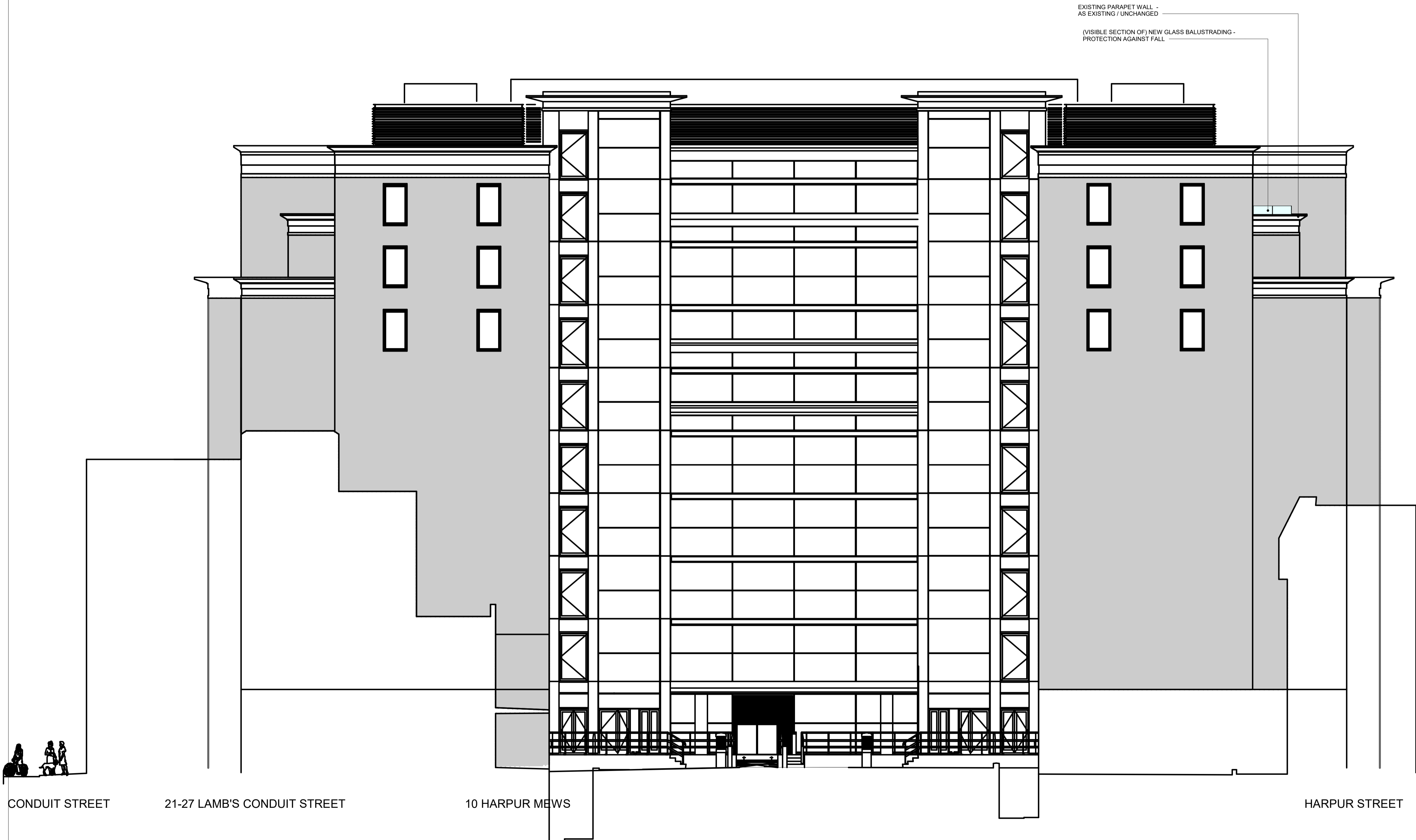
1 North Elevation as Proposed 1 : 100
