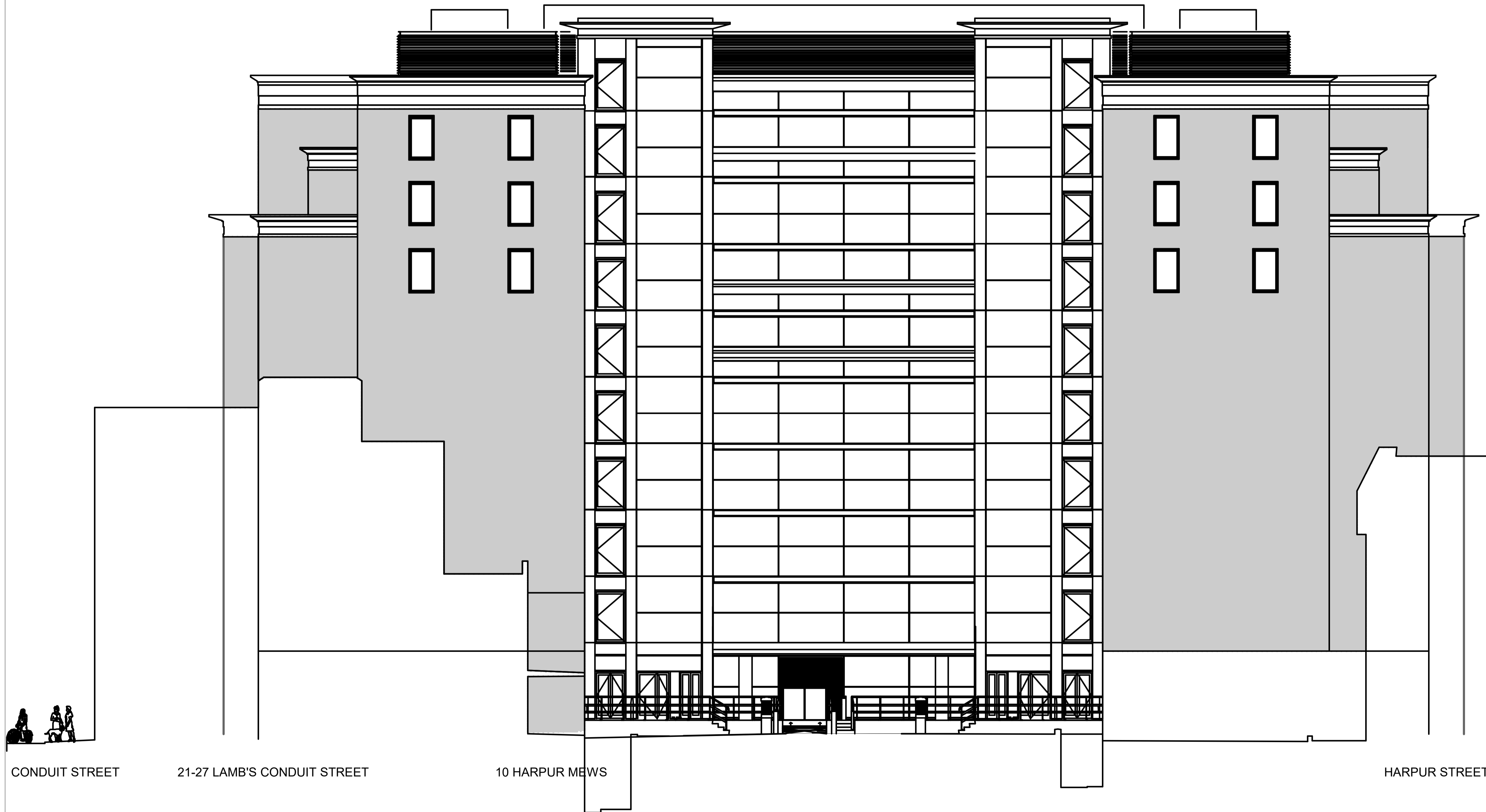
1 North Elevation as Existing 1 : 100
