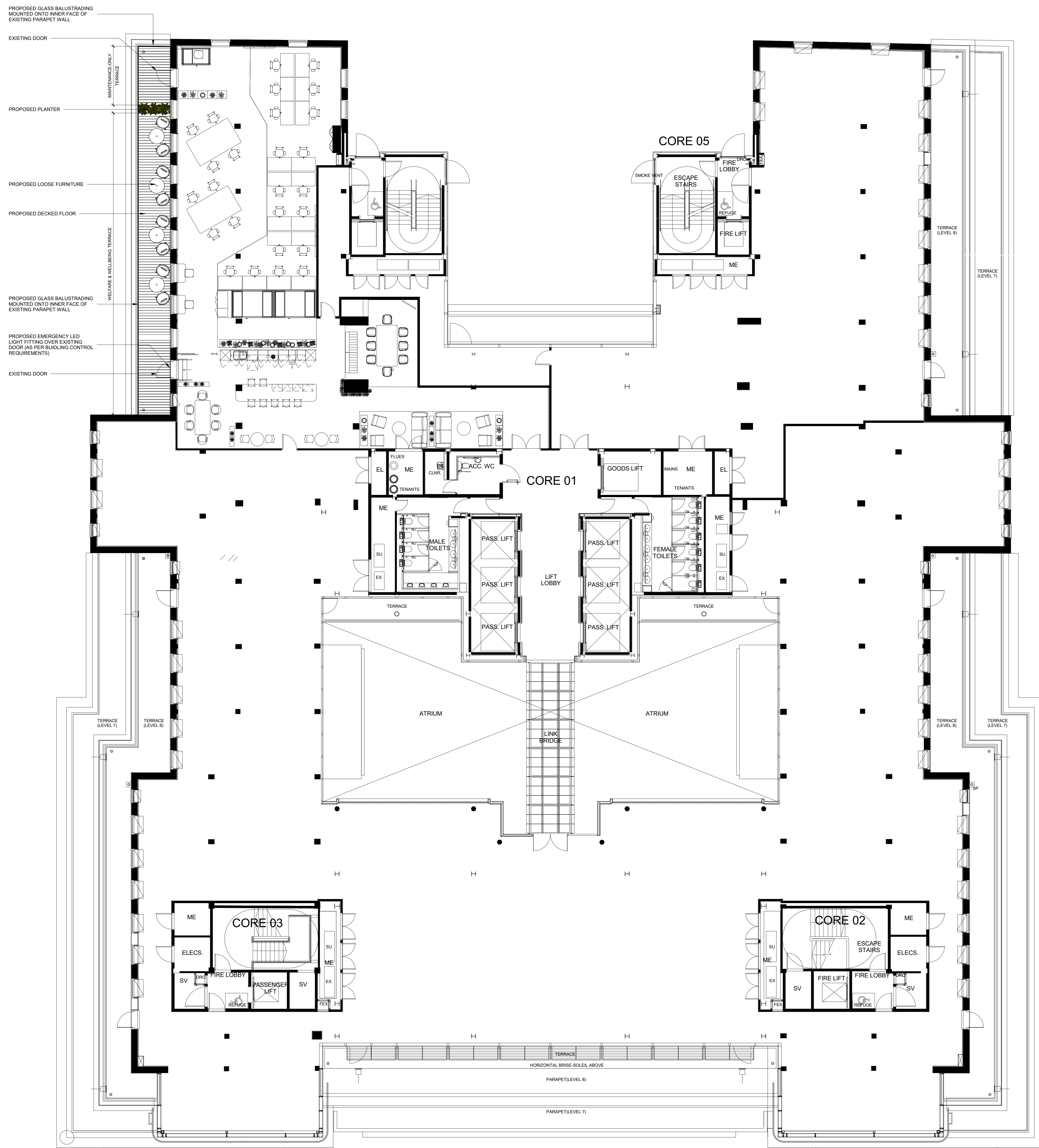
1 Proposed Floor Plan 1:100
