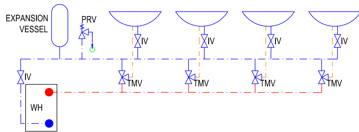
TYPICAL WASH HAND BASIN SCHEMATIC
