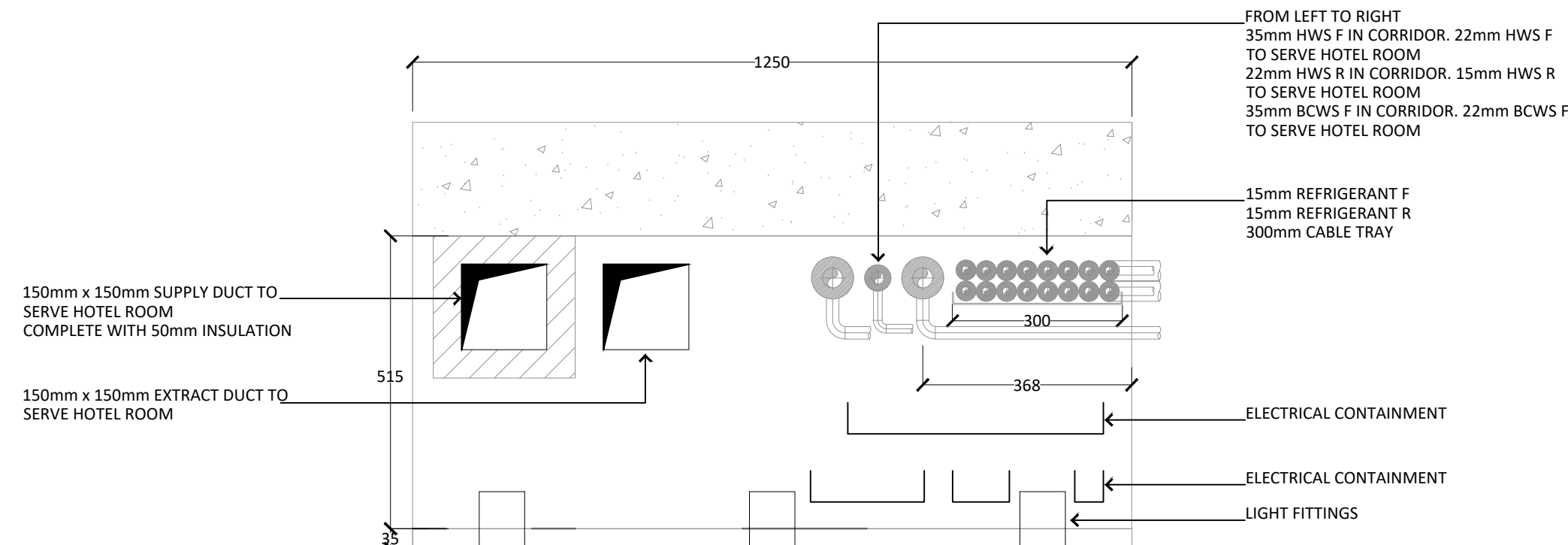
SECTION G-G (1:10)
