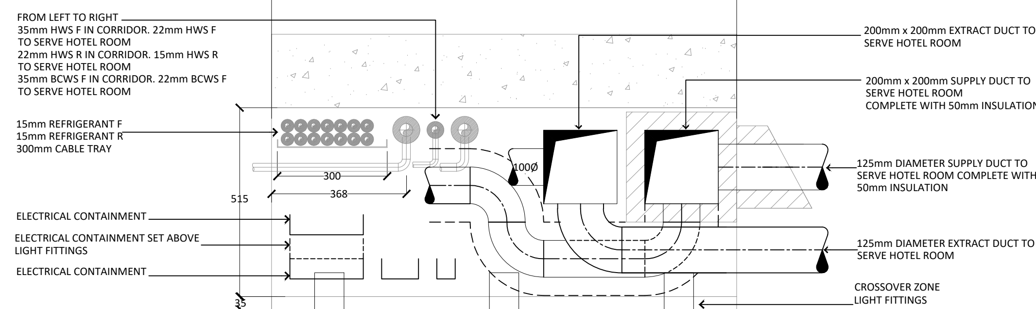
SECTION D-D (1:10)
