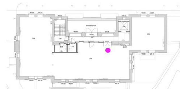
FLOOR PLAN
