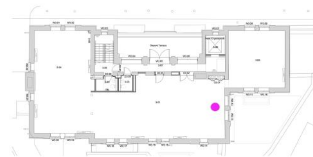
FLOOR PLAN
