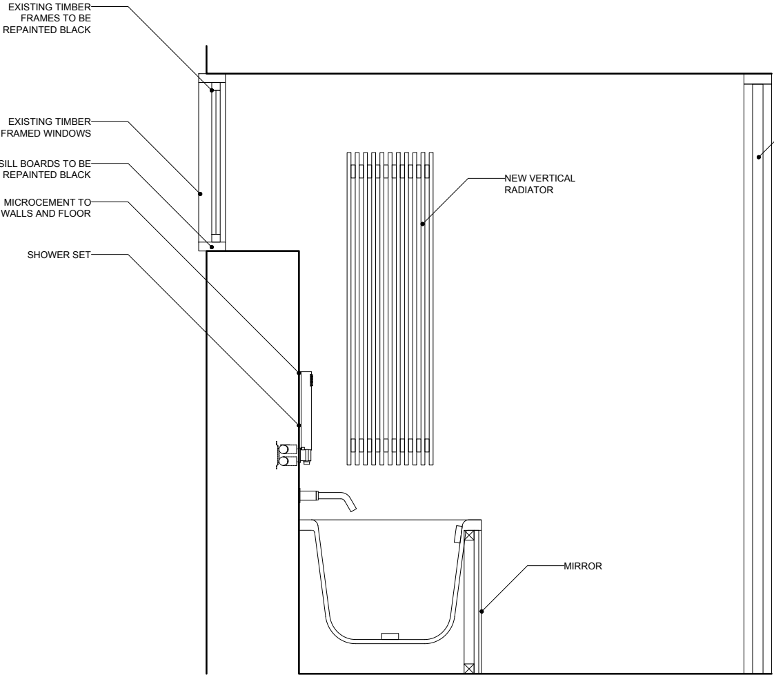
BATHROOM ELEVATION A
