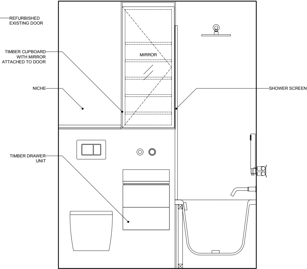
BATHROOM ELEVATION B
