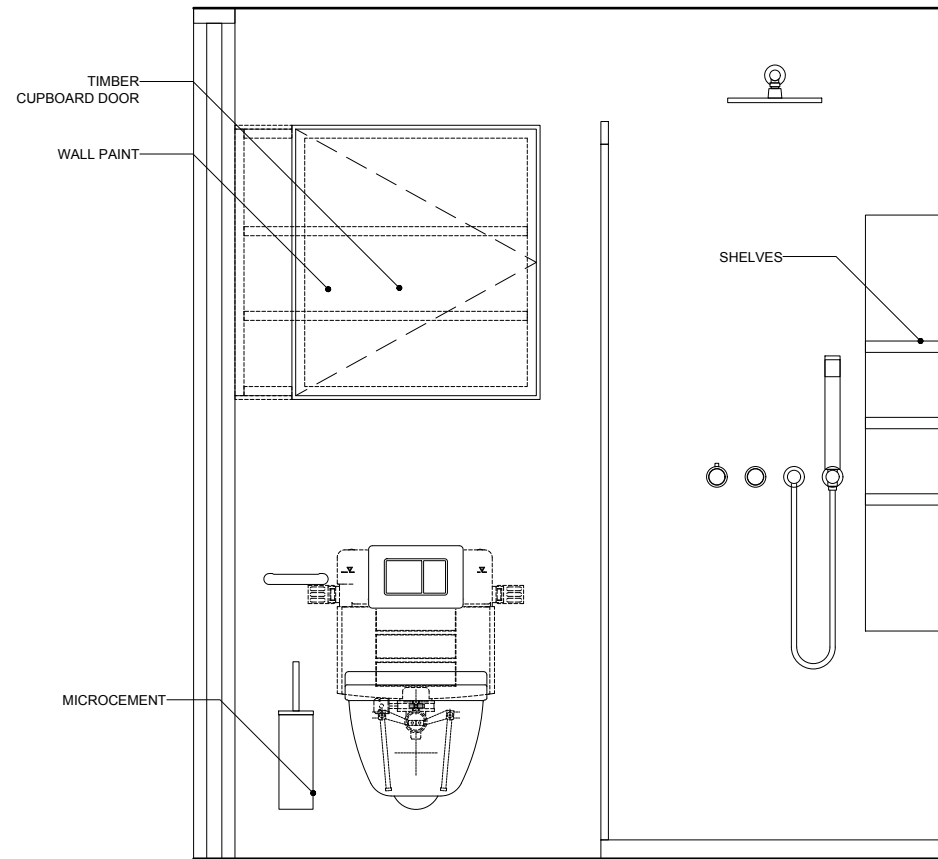
SHOWER ROOM ELEVATION C
