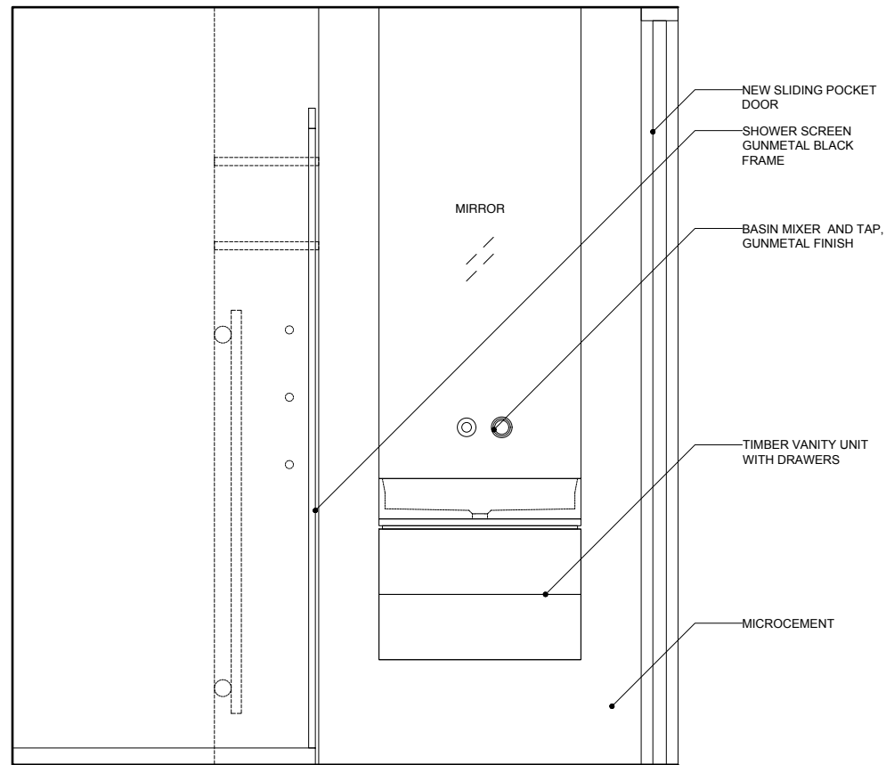
SHOWER ROOM ELEVATION D
