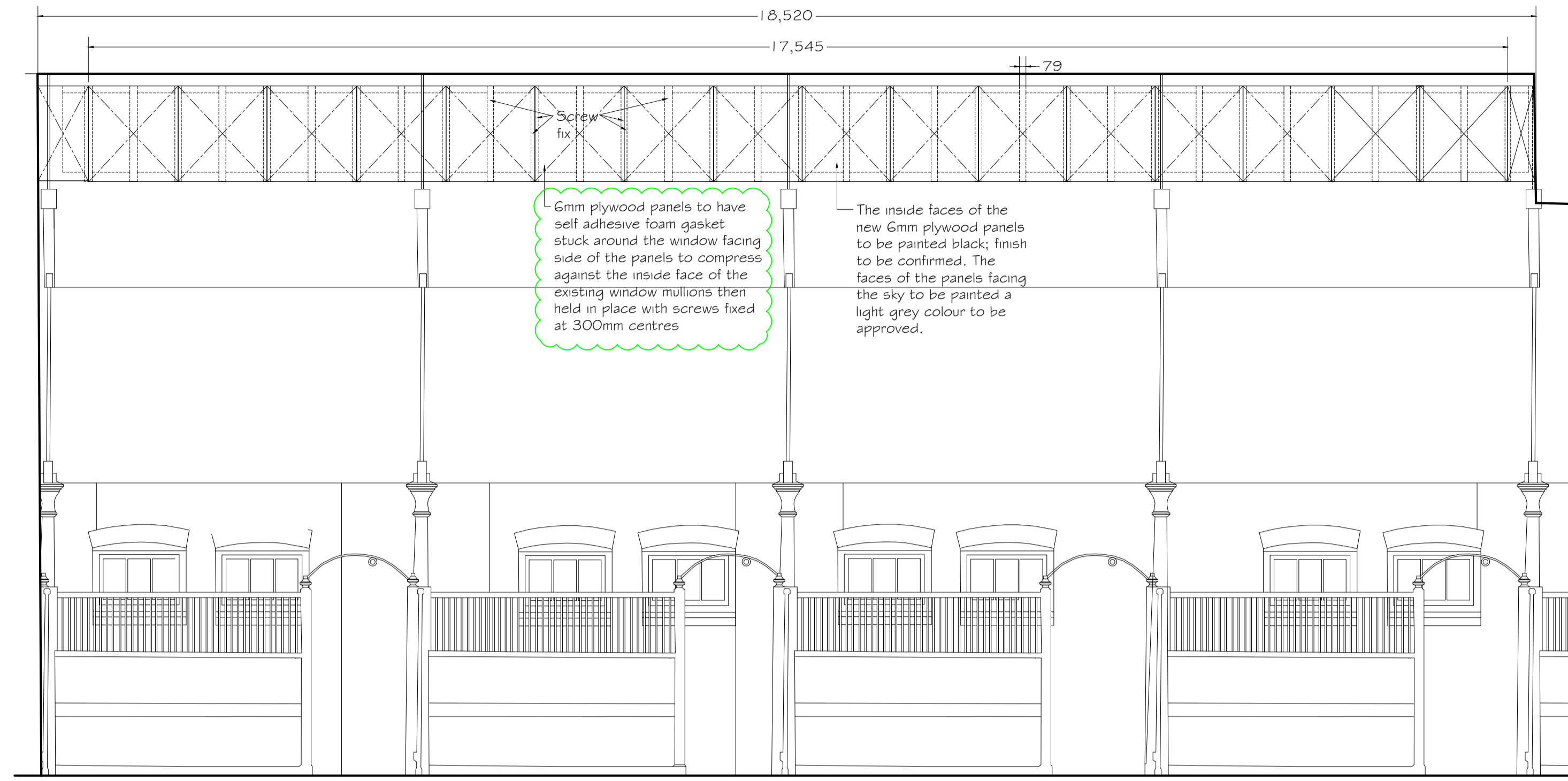
ELEVATION 1.50 scale NB: The mirror image of the above to be applied to the opposite elevation.
