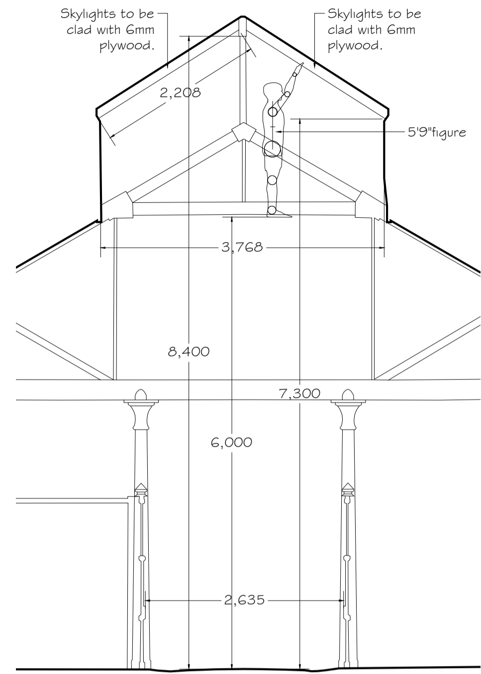
SECTION 1.50 scale
