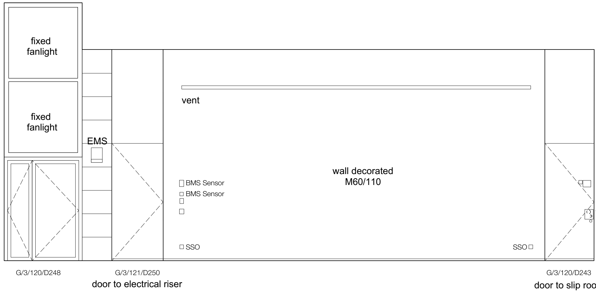
Elevation 3 - West Wall
