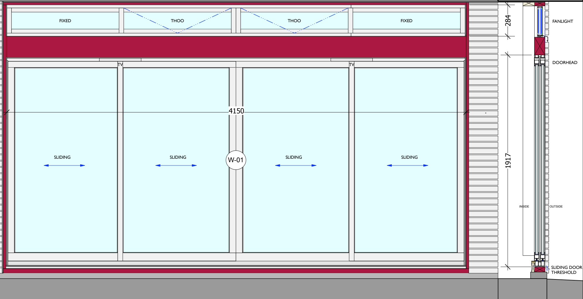
SLIDING DOOR ELEVATION TO FLATS 15 & 16. (W-01 ON PLAN)
