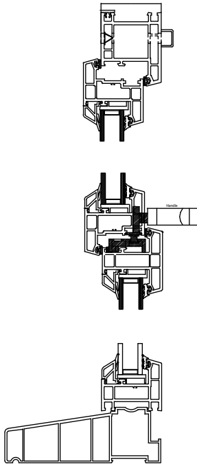
WINDOW SILL, TRANSOM & HEAD 1:5
