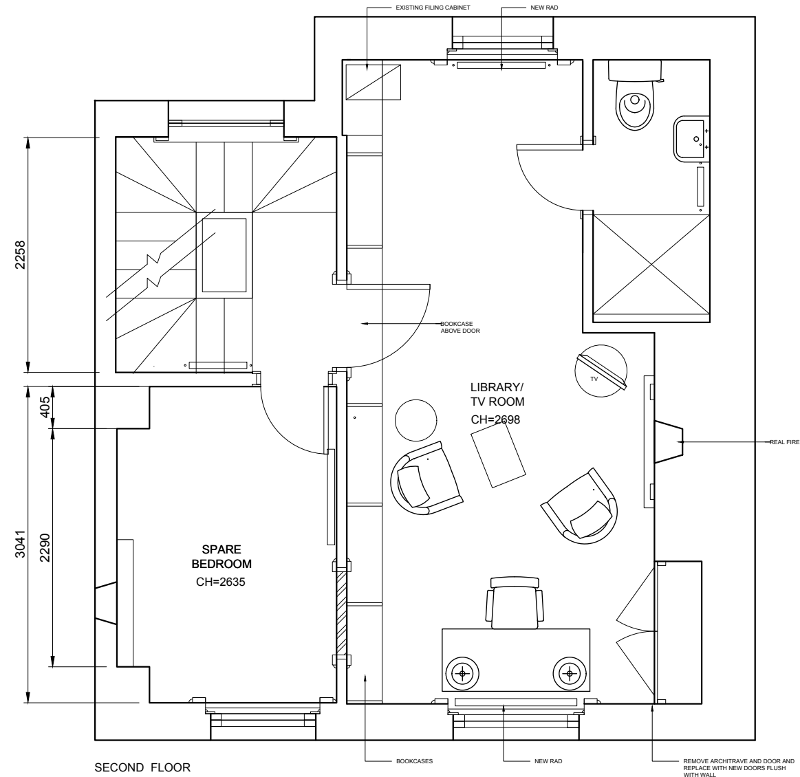
SECOND FLOOR
