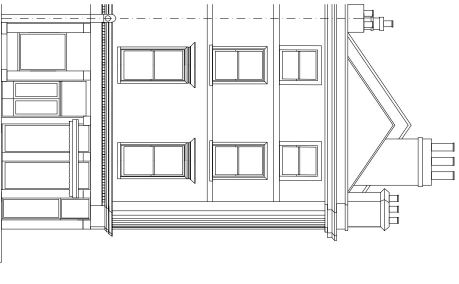
WEST ELEVATION AS EXISTING
