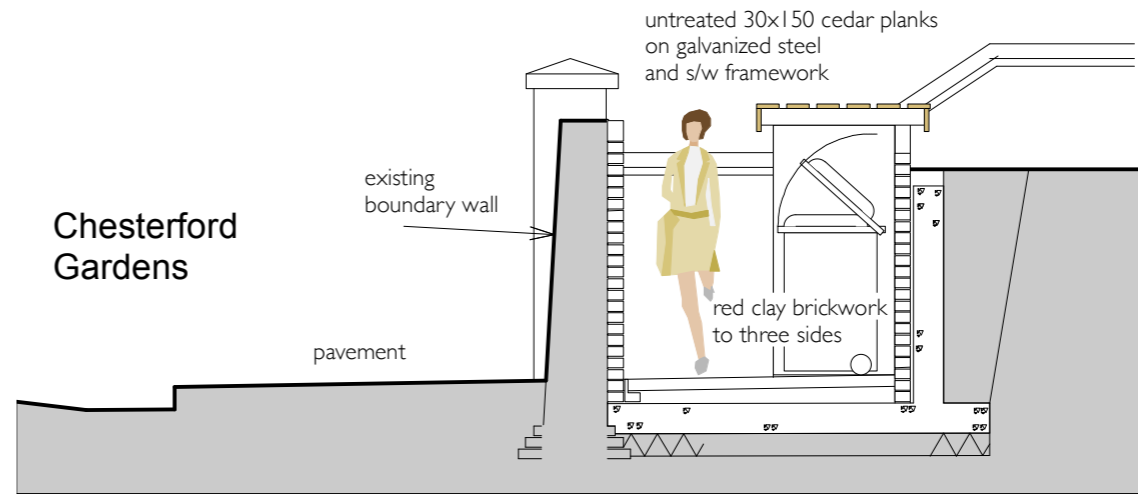
2 Cross Section B-B
