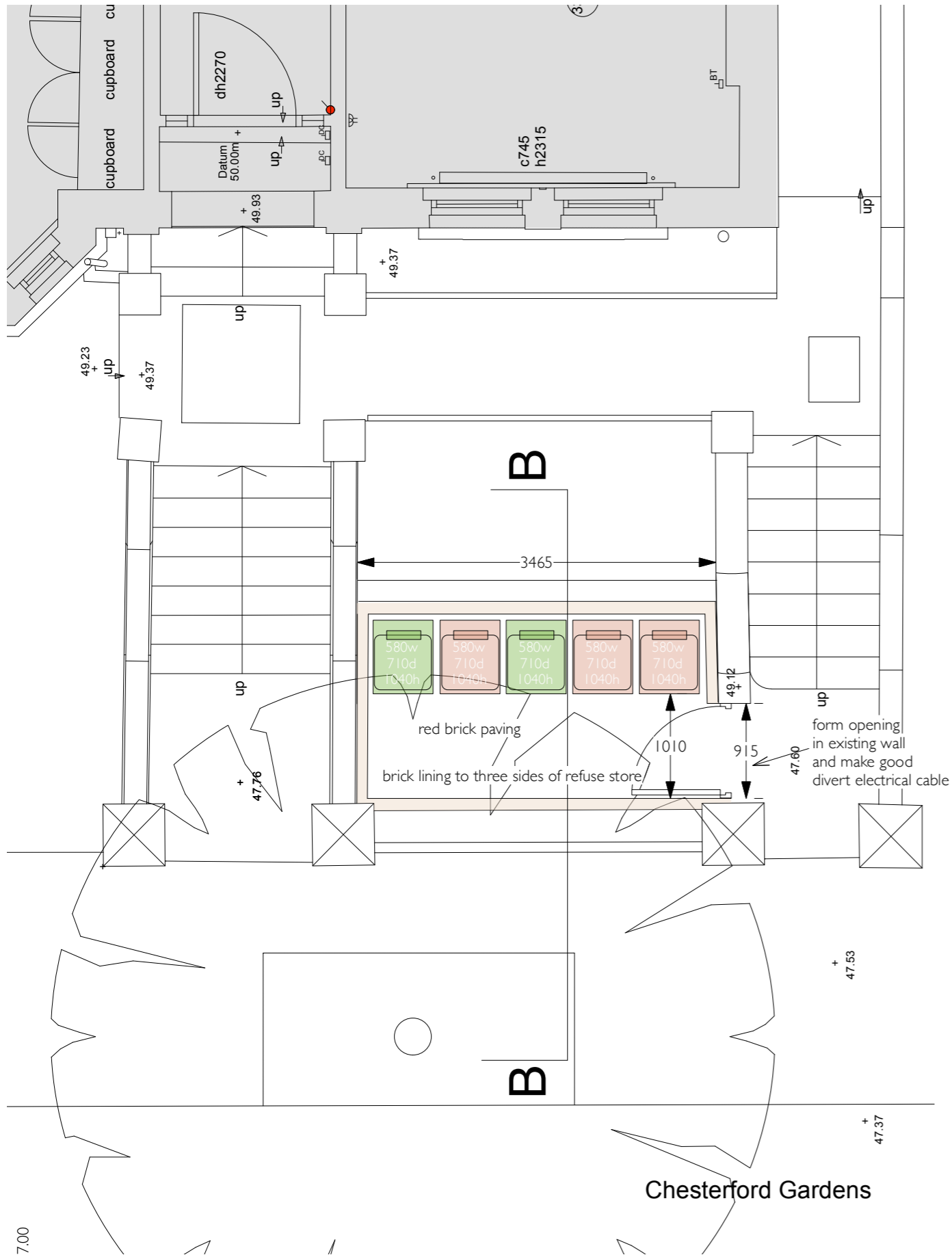
1 Plan of Refuse Store
