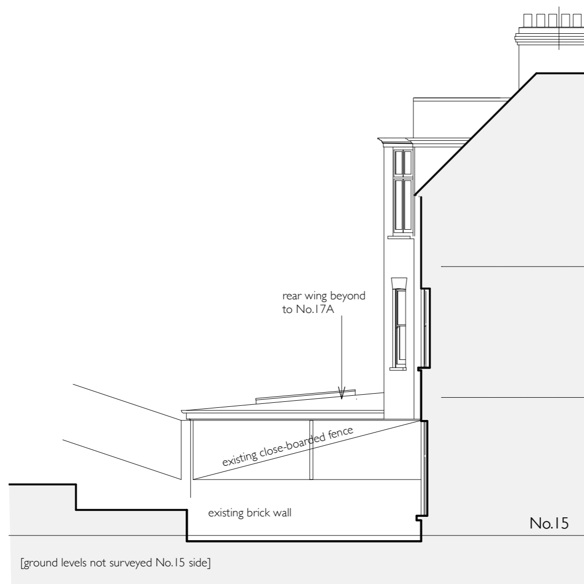
1 North Elevation As Proposed - As seen from No. 15 Scale 1:100
