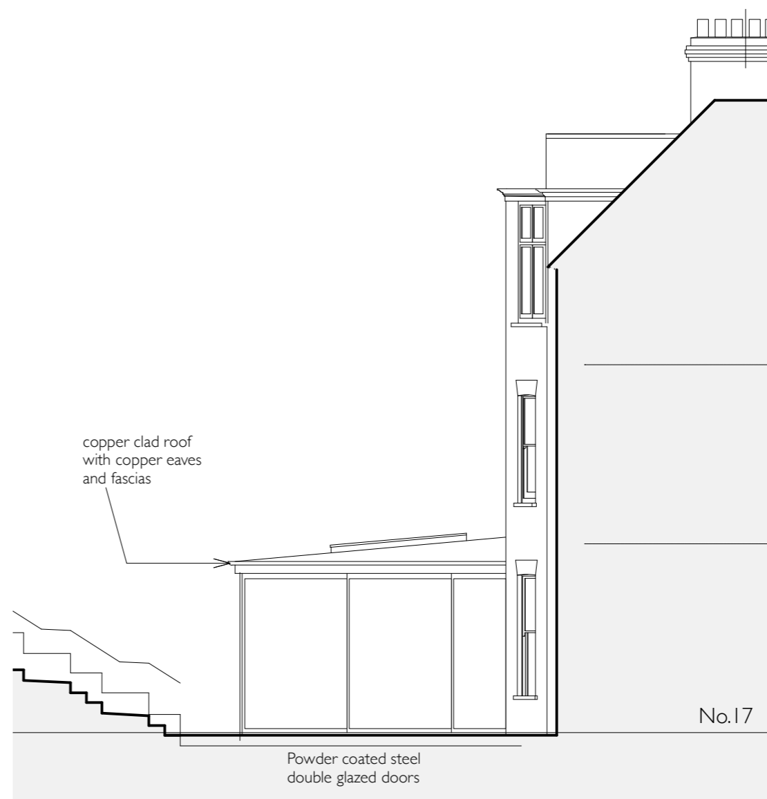
2 North Elevation of New Extension As Proposed Scale 1:100
