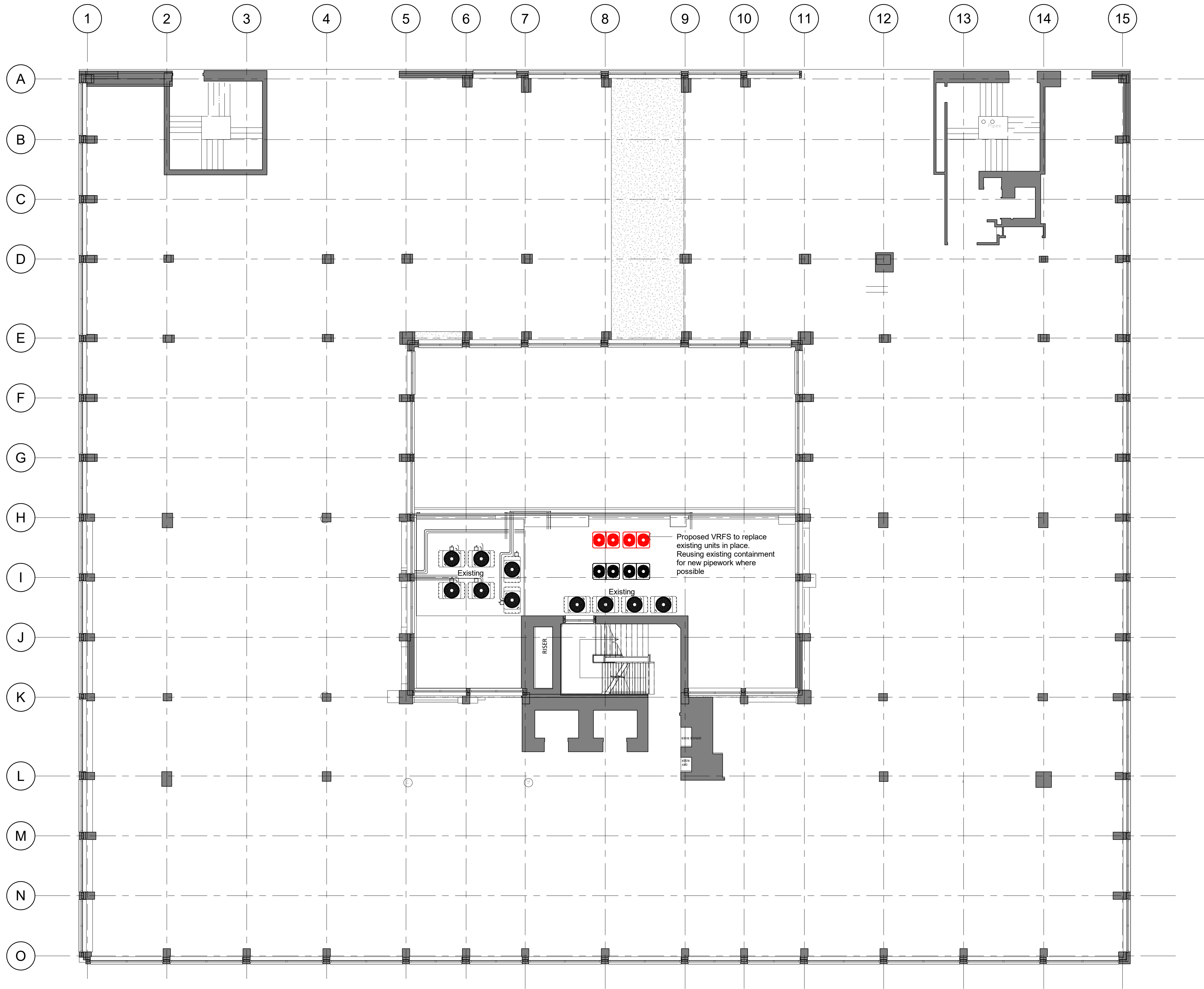
1 Proposed First Floor Condenser Unit 1 : 100
