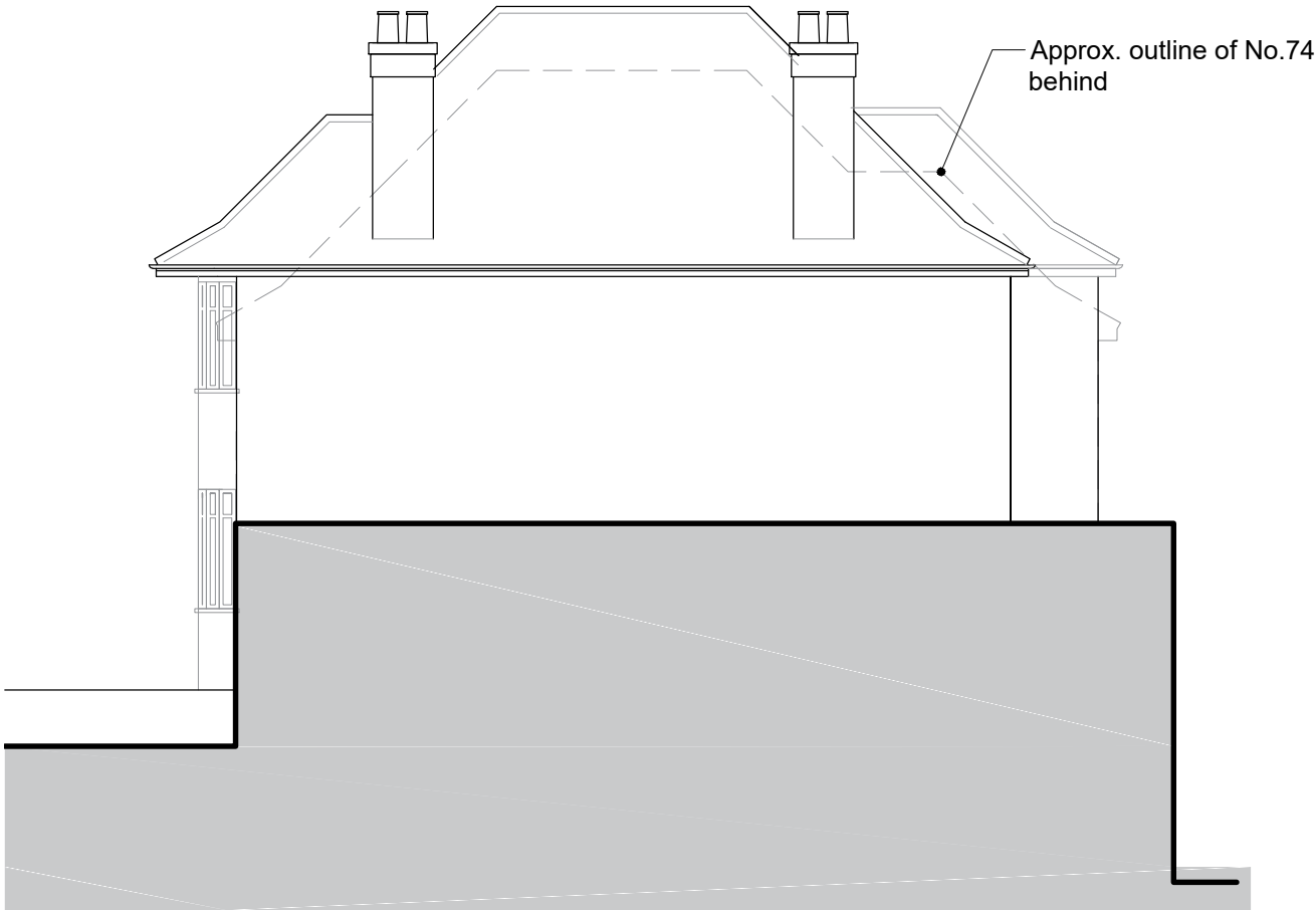
2. EXISTING SOUTH ELEVATION
