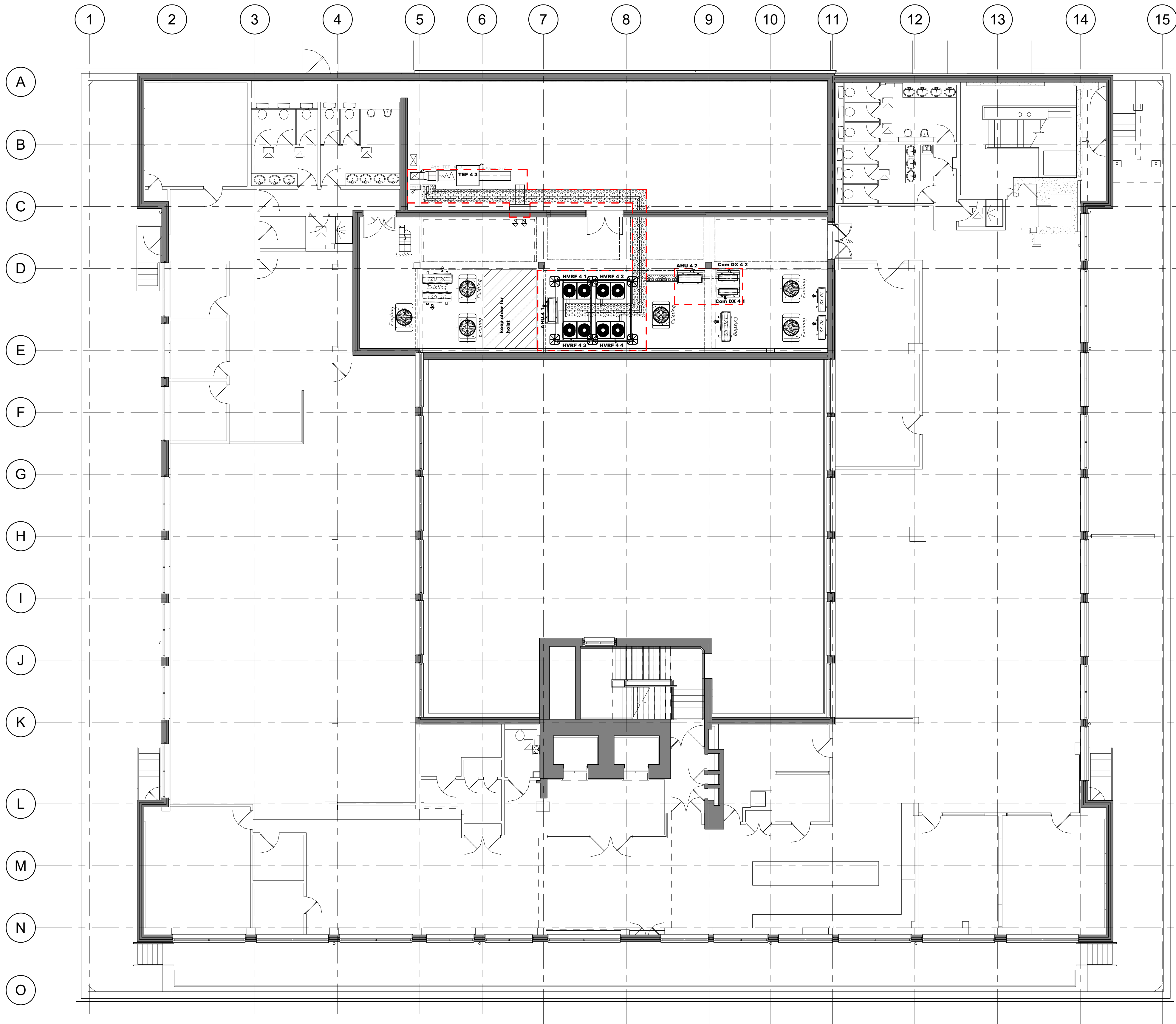
1 Proposed Fifth Floor Condenser Location 1 : 100
