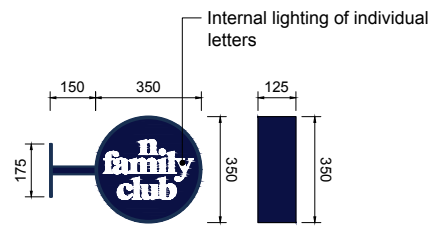
PROJECTING SIGN ELEVATION DETAILS 1:25 @ A3
