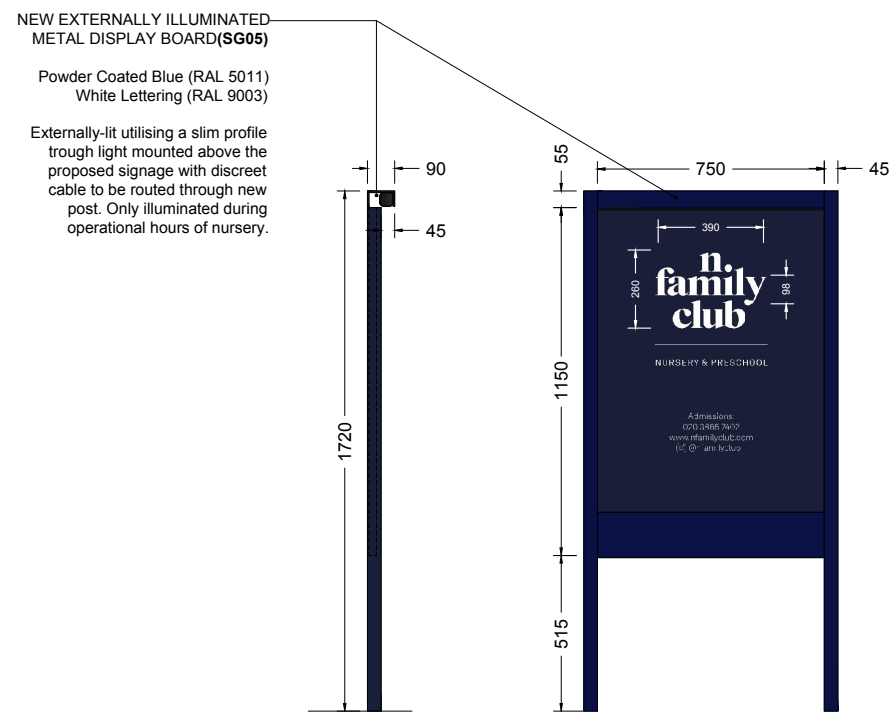
DISPLAY BOARD ELEVATION & SECTION DETAILS 1:25 @ A3
