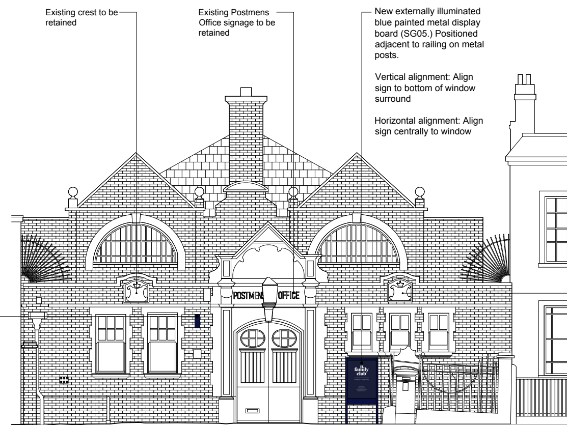
PROPOSED STREET ELEVATION 1:100@A3
