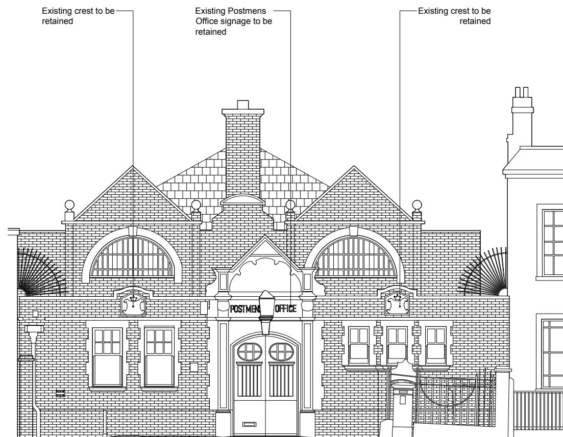
EXISTING STREET ELEVATION 1:100@A3
