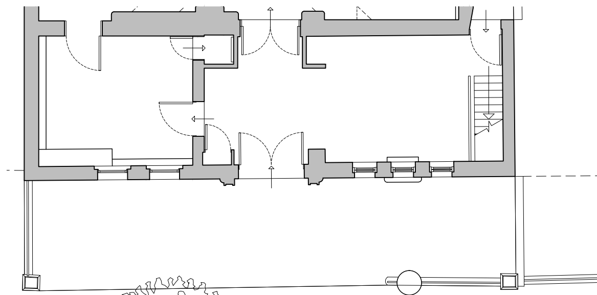
EXISTING PLAN 1:100 @ A3
