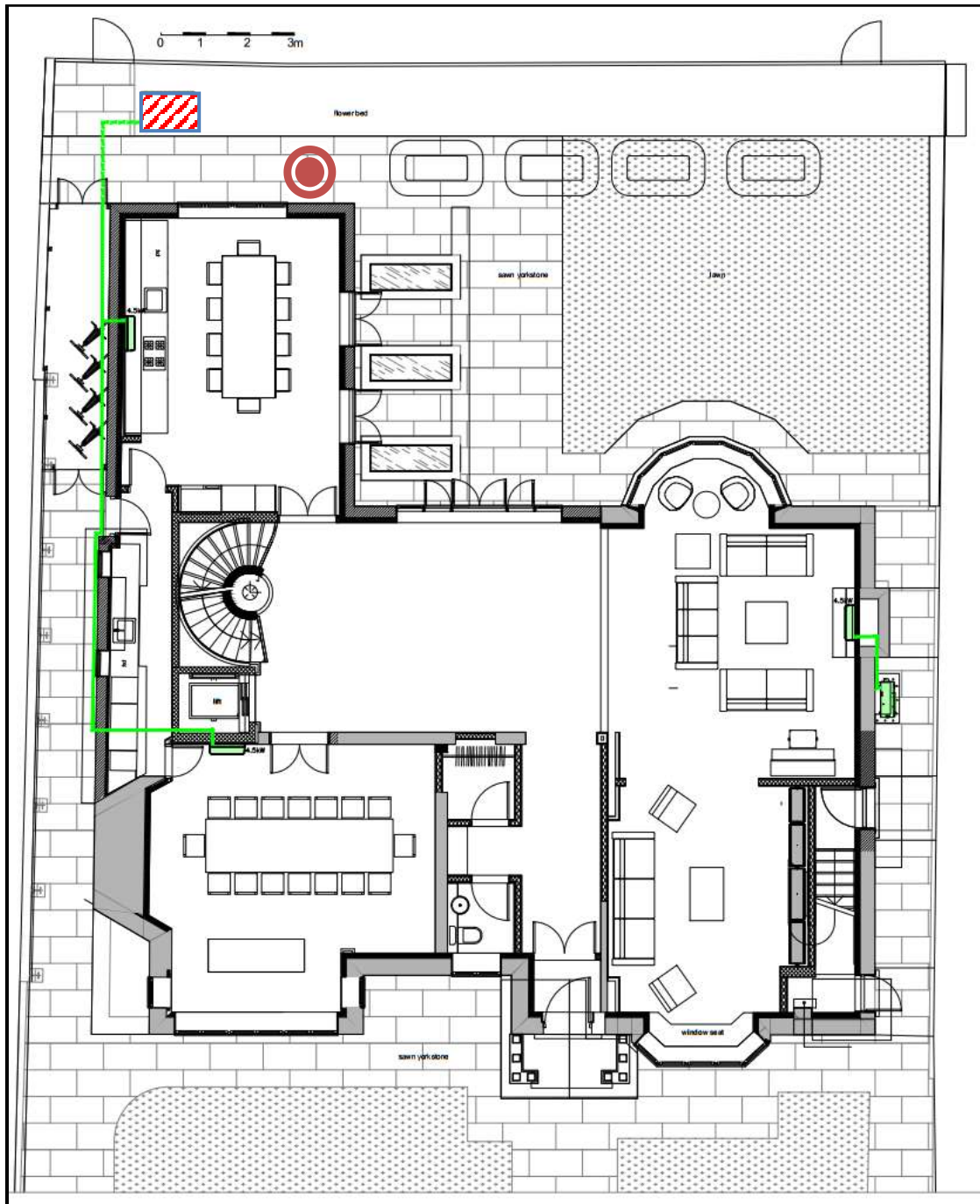
Figure 2.2 Site measurement position and proposed plant unit installation (Drawing source: Nationwide Heating & Cooling Ltd.)
