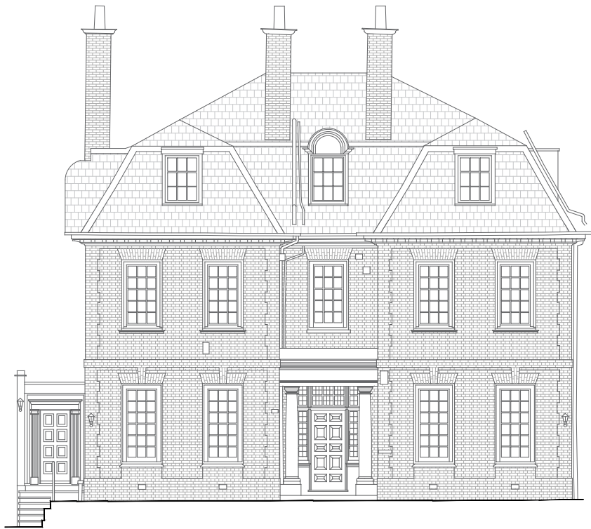
EXISTING WEST ELEVATION (PRINCIPLE ELEVATION)
