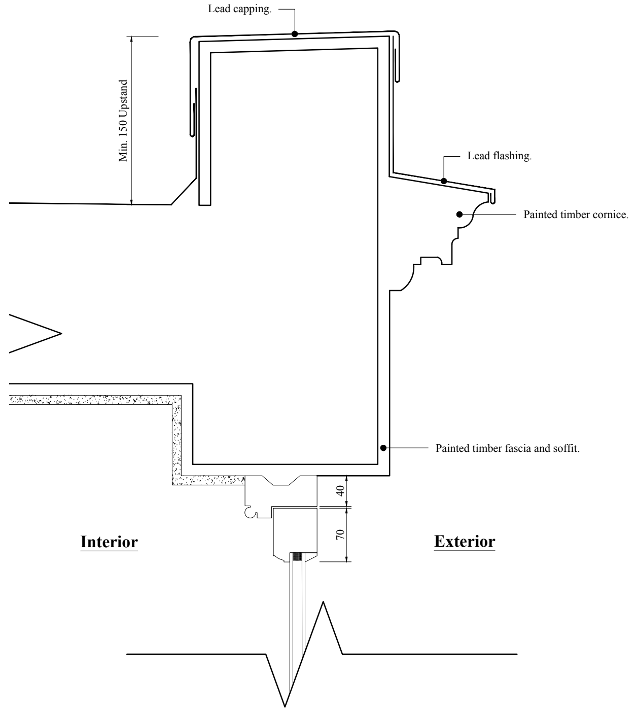
Proposed Parapet and Patio Doors Head
