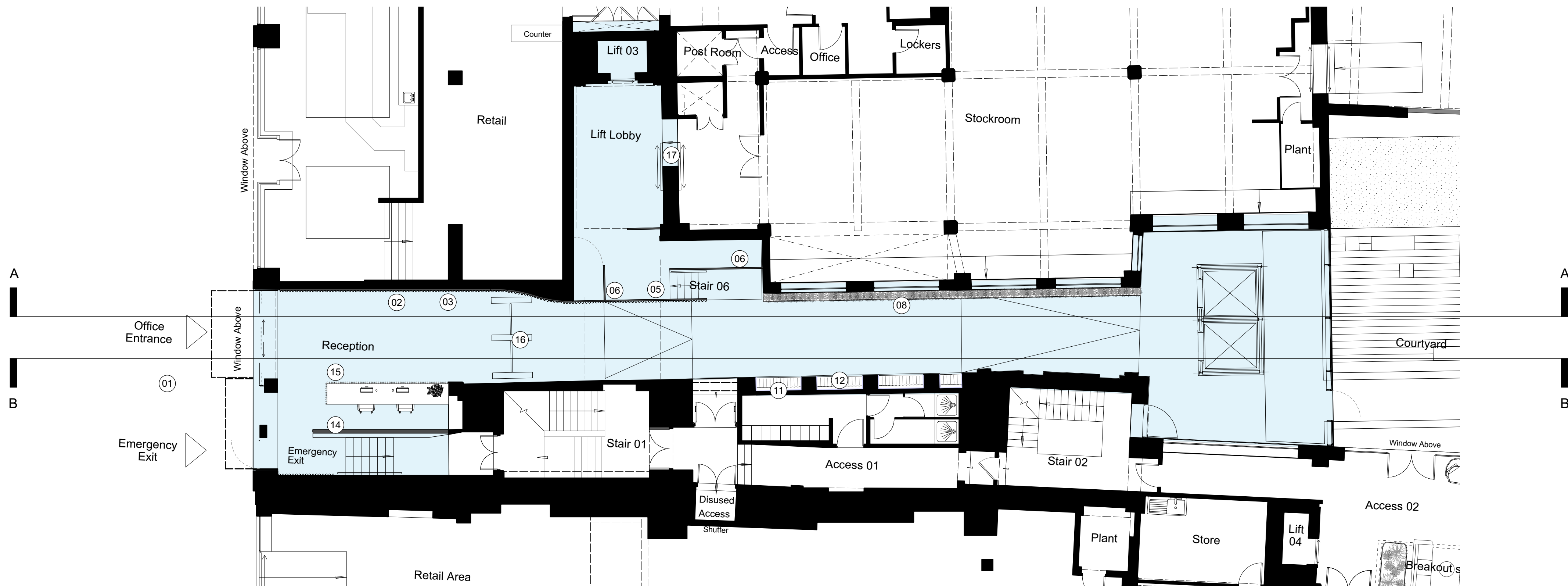
01 Proposed Torrington Place Reception Plan Scale: 1:100
