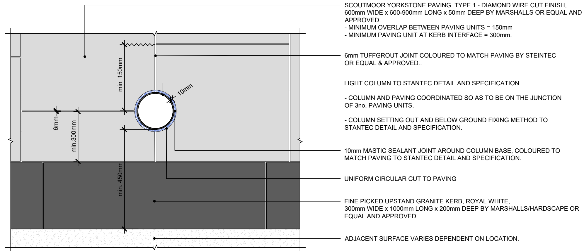
16 TYPICAL DETAIL PLAN ON HIGHWAY LIGHTING COLUMN SCALE: 1:10 @ A3
