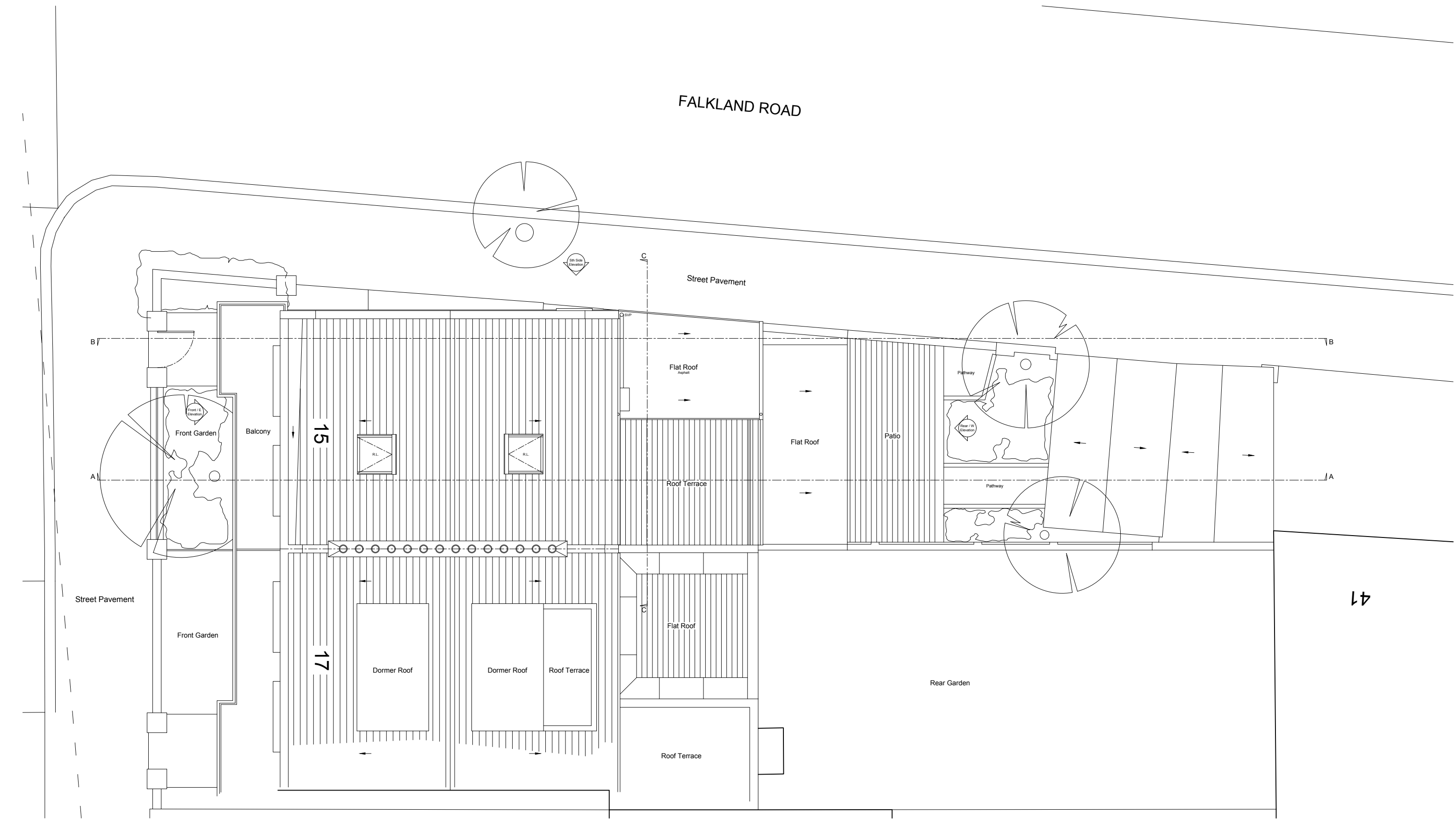
PROPOSED ROOF PLAN - NO CHANGE 1:100
