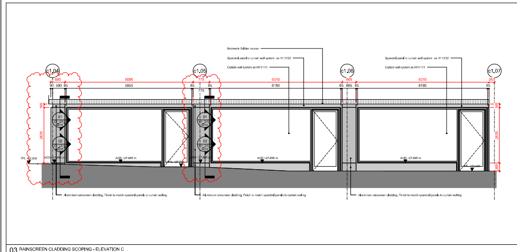
03 RAINSCREEN CLADDING SCOPING - ELEVATION C
