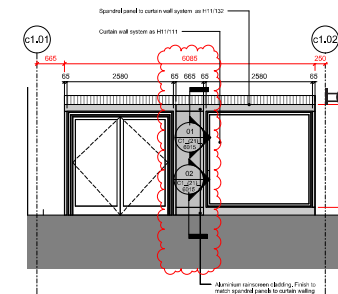
04 RAINSCREEN CLADDING SCOPING - ELEVATION D
