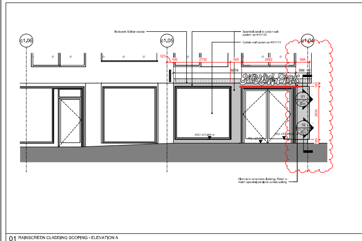
01 RAINSCREEN CLADDING SCOPING - ELEVATION A
