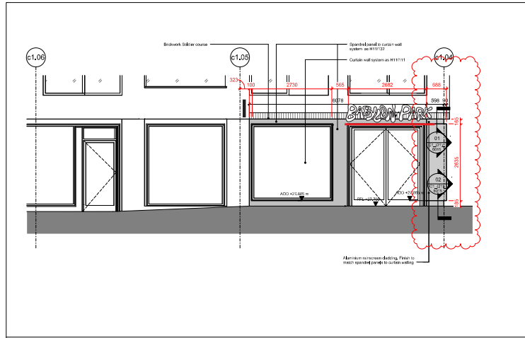
01 RAINSCREEN CLADDING SCOPING - ELEVATION A
