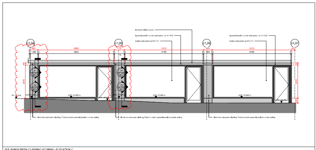
03 RAINSCREEN CLADDING SCOPING - ELEVATION C
