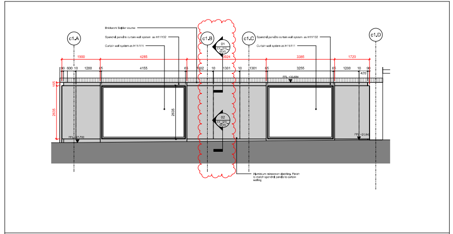
02 RAINSCREEN CLADDING SCOPING - ELEVATION B
