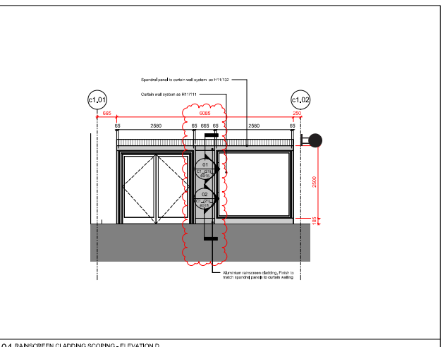
04 RAINSCREEN CLADDING SCOPING - ELEVATION D
