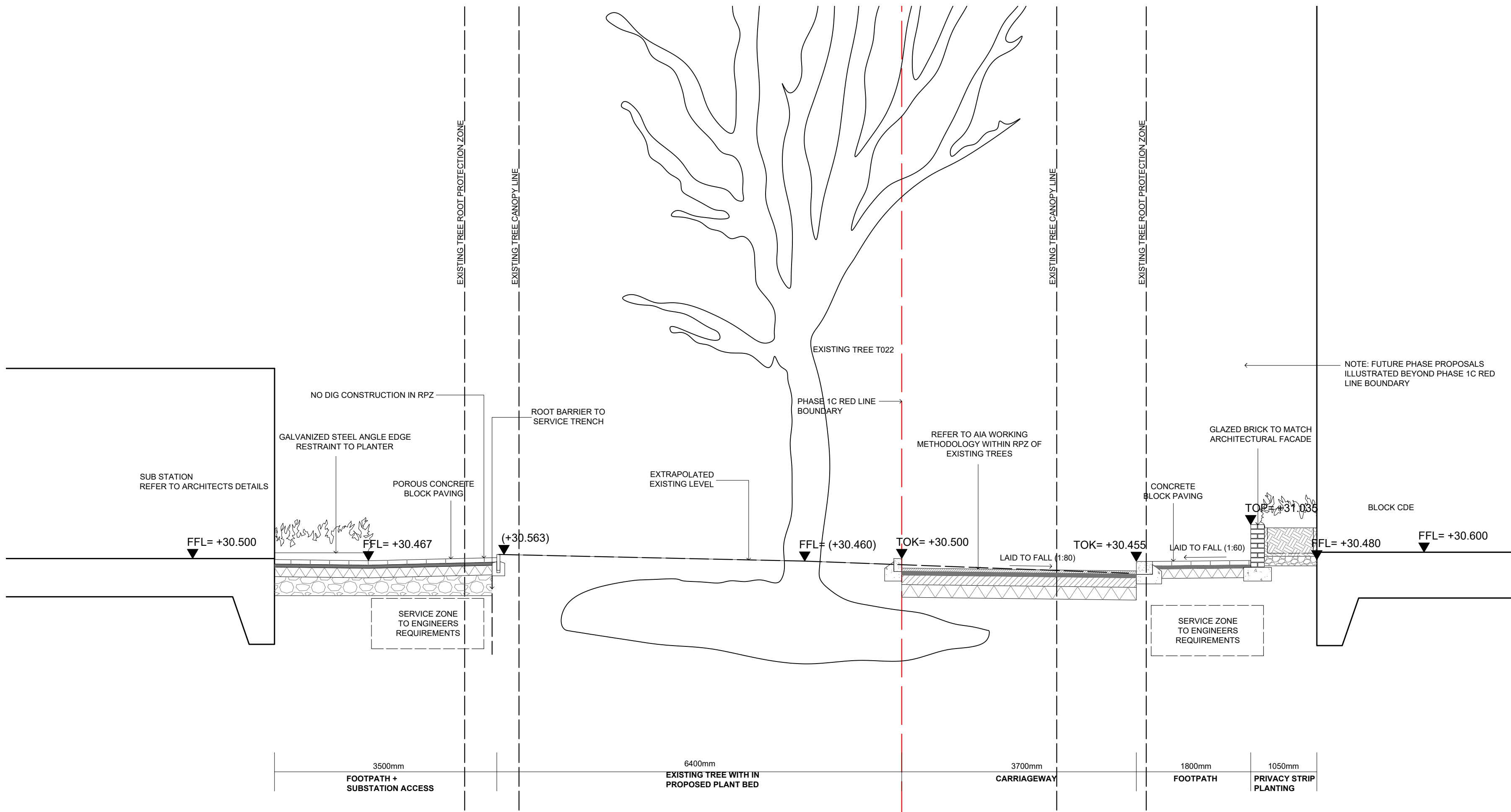
1 SECTION A-A' REF T022 SCALE 1:50
