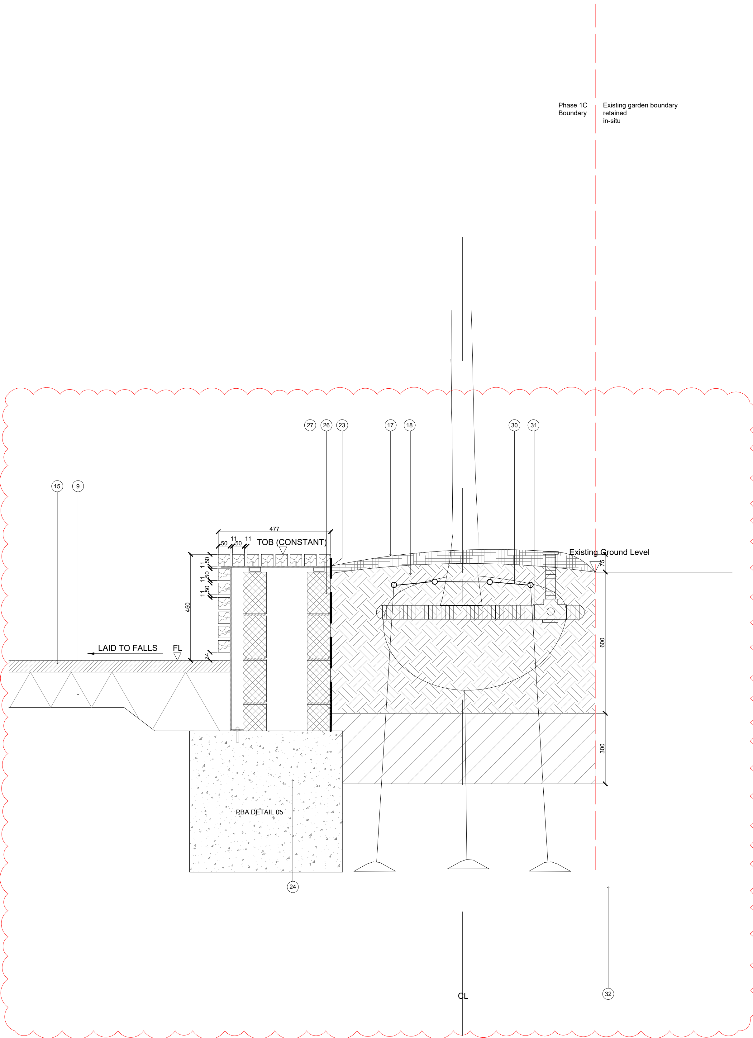
2 RAISED PLANTER BENCH TYPE B3 TO PLOT J,K & L COURTYARD ALLOTMENT GARDEN SCALE 1:10
