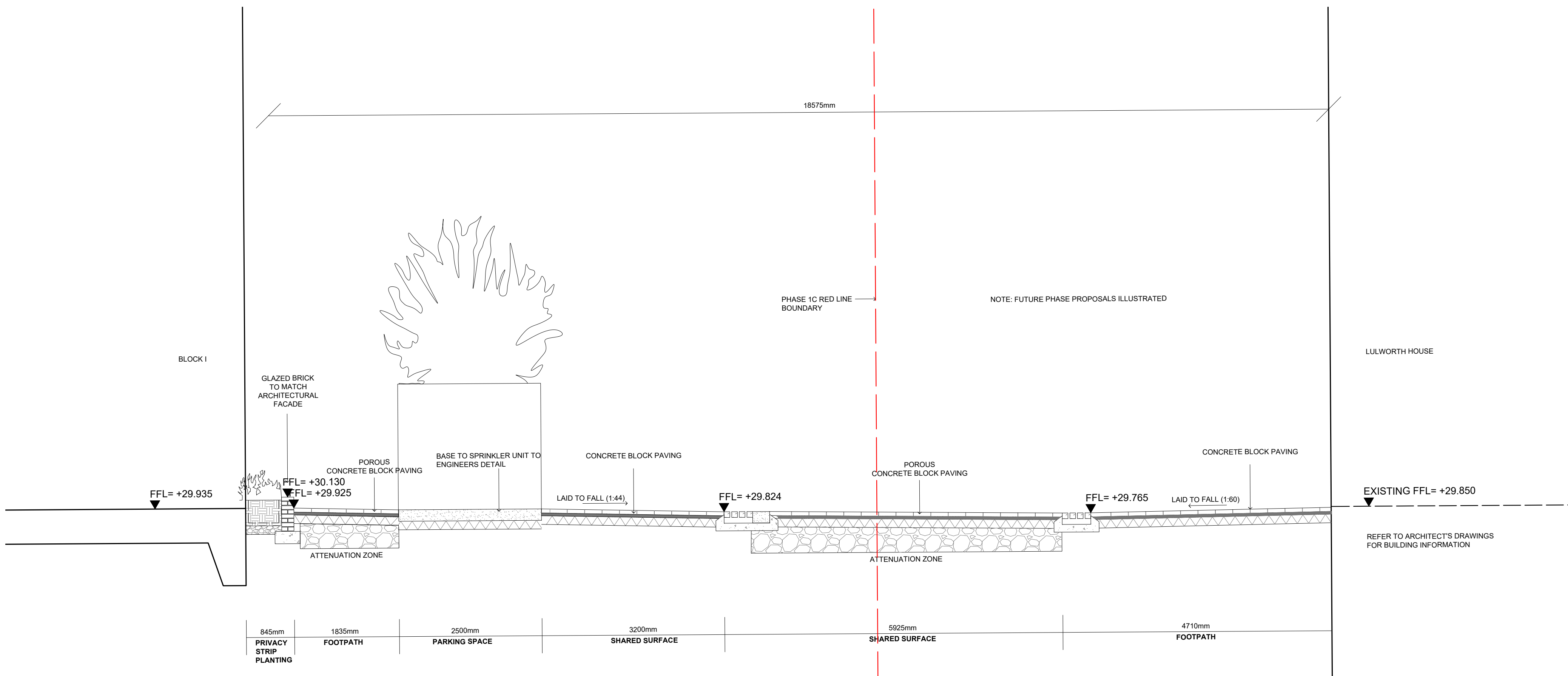
2 SECTION B-B' SCALE 1:50
