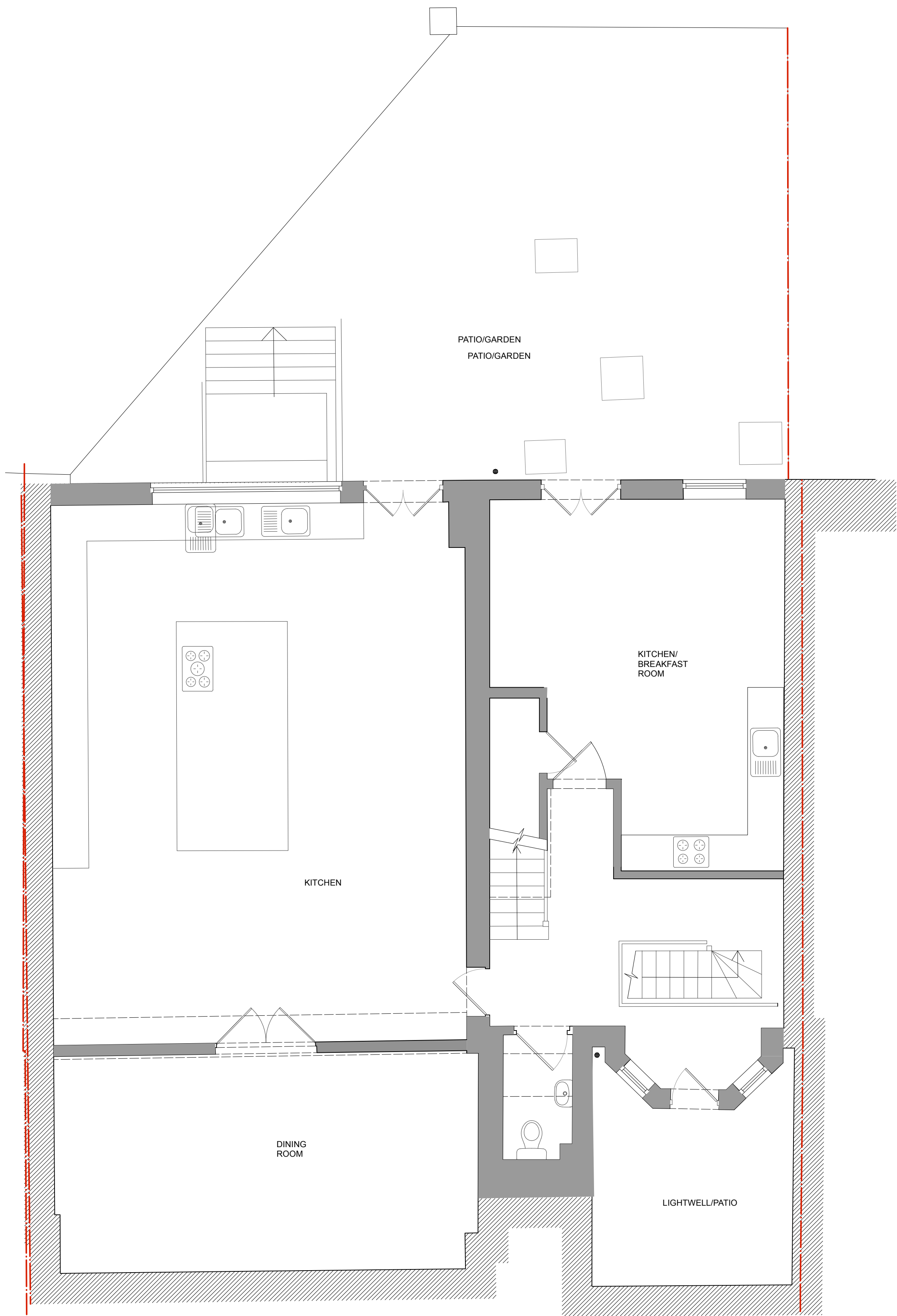
BASEMENT
