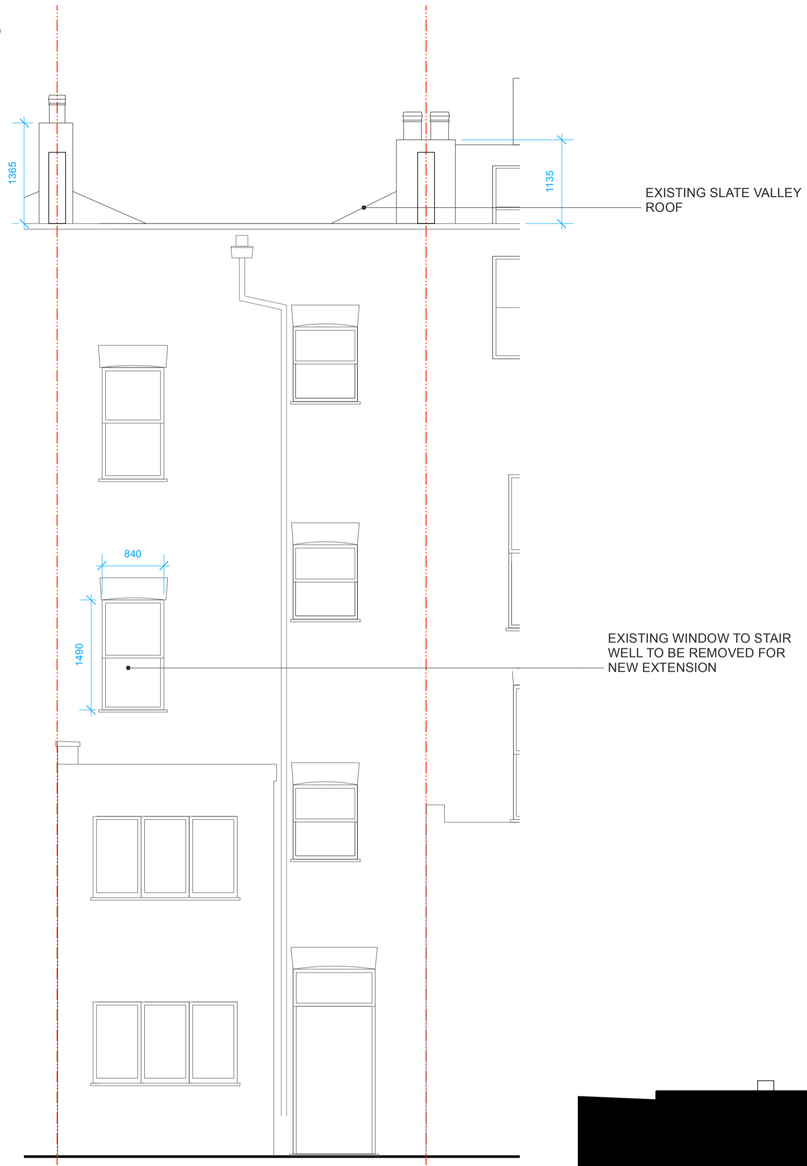
4 Rear Elevation 1:50
