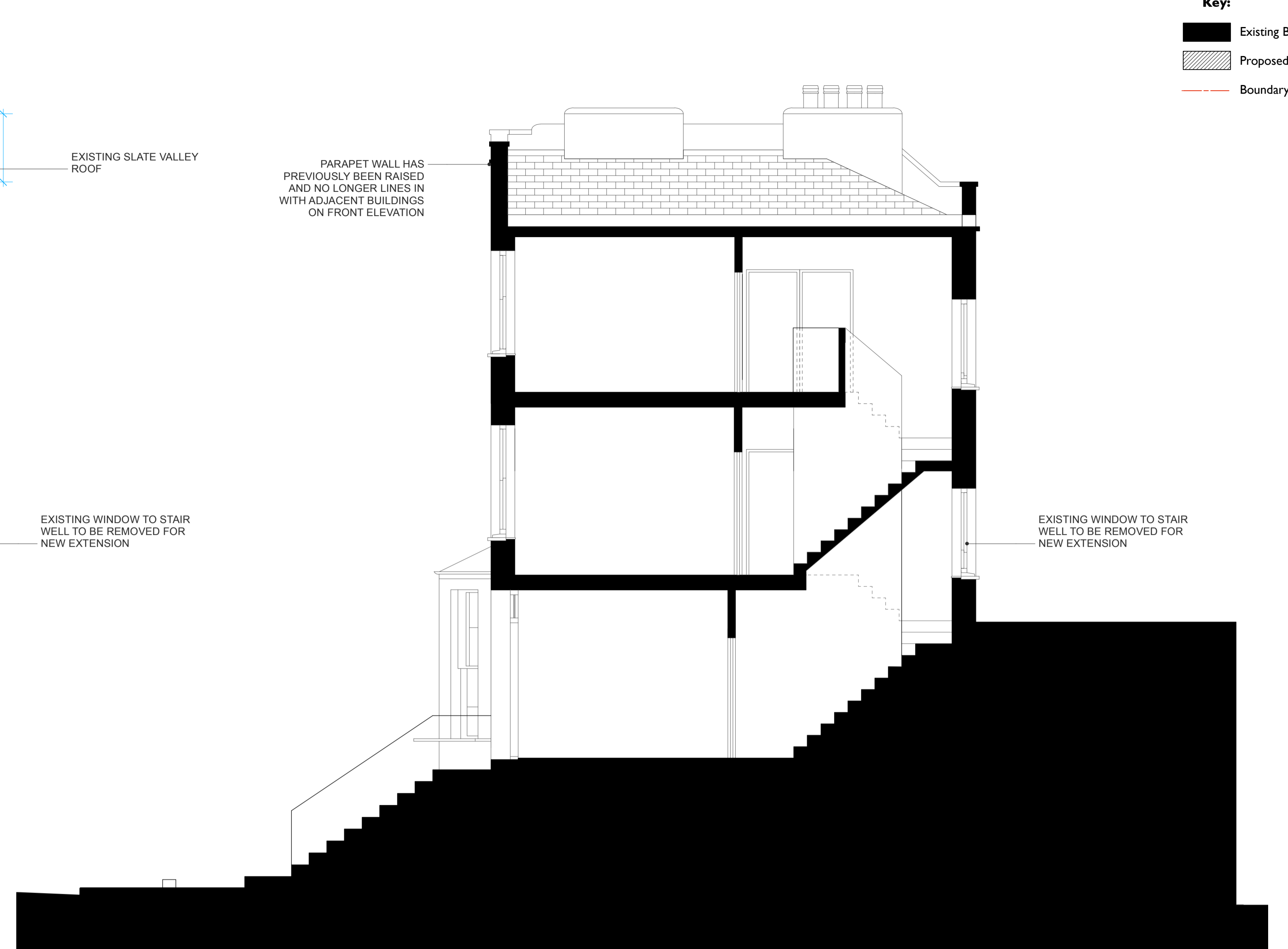
8 Section AA 1:50
