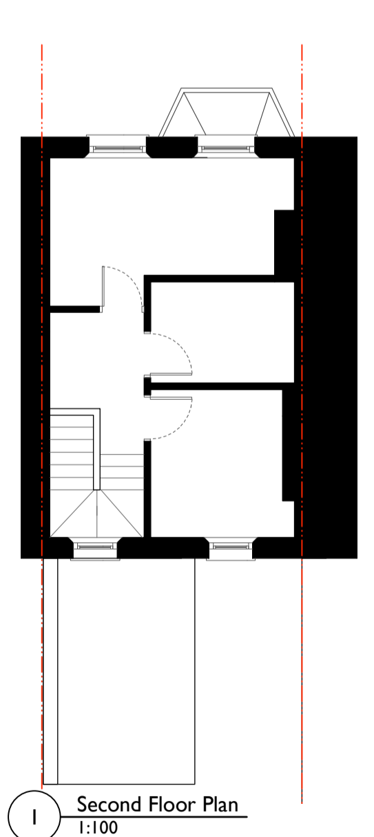
1 Second Floor Plan 1:100
