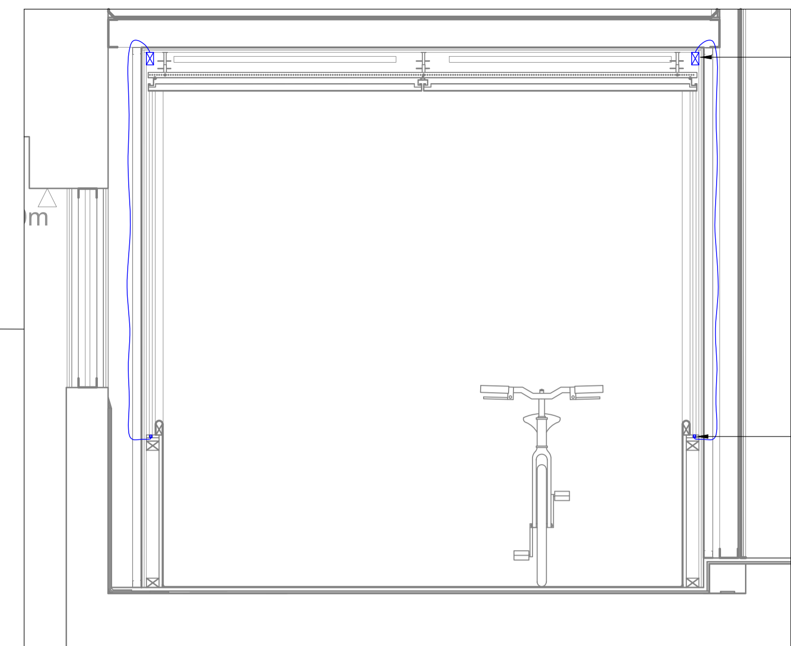
Indicative Section Through Tunnel 1:20 @A1
