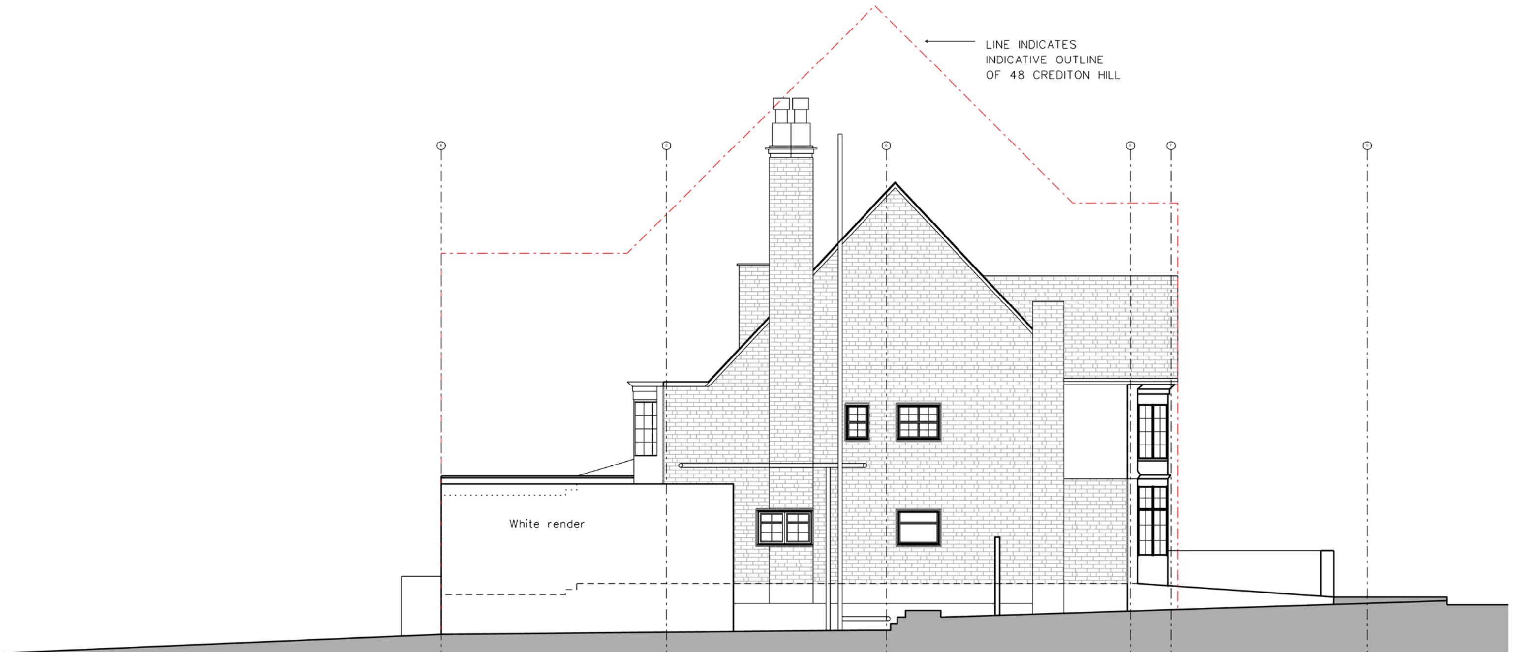
① Side Elevation Existing 1:100
