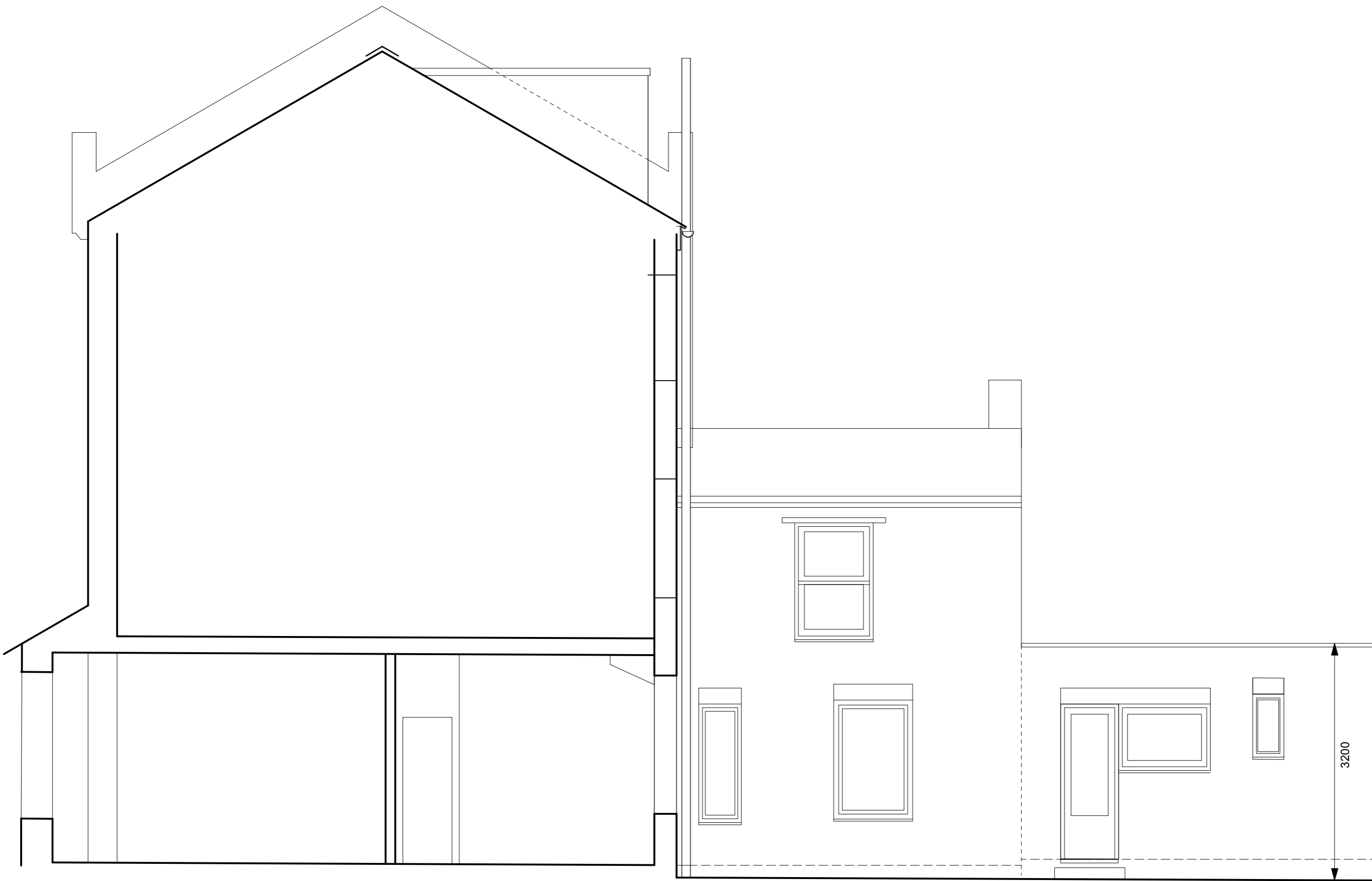
SIDE ELEVATION EXISTING
