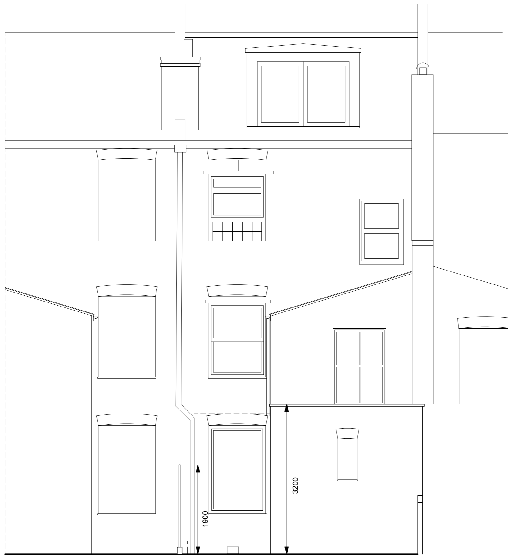
REAR ELEVATION EXISTING
