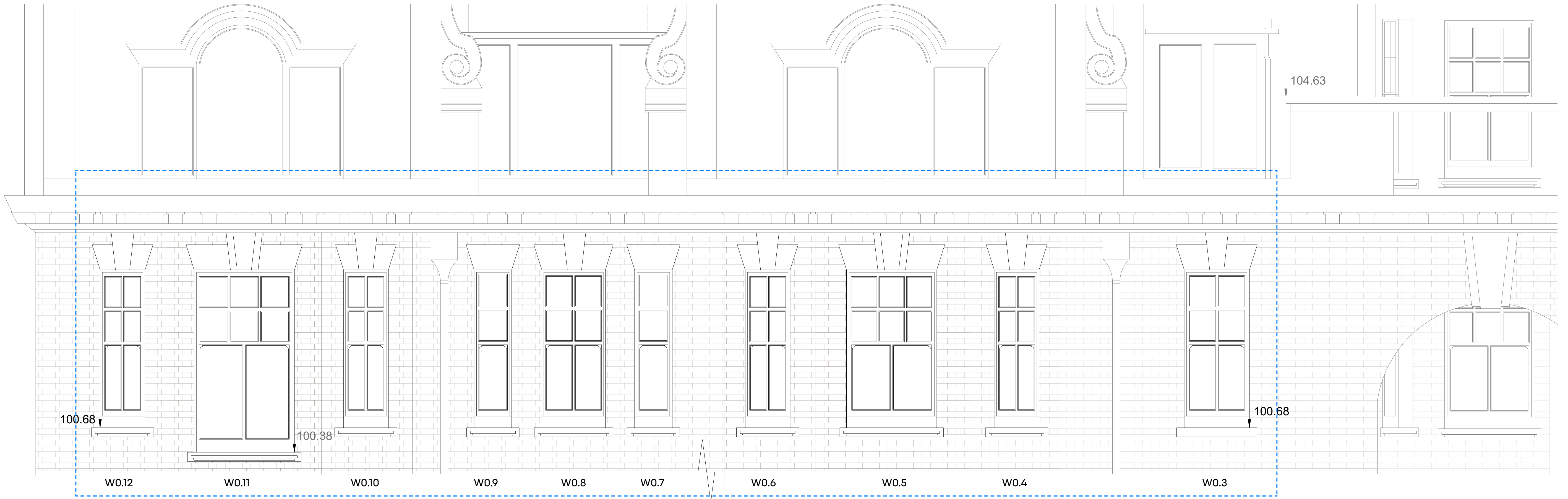
1 Proposed North-East Elevation 1:25 @A1
