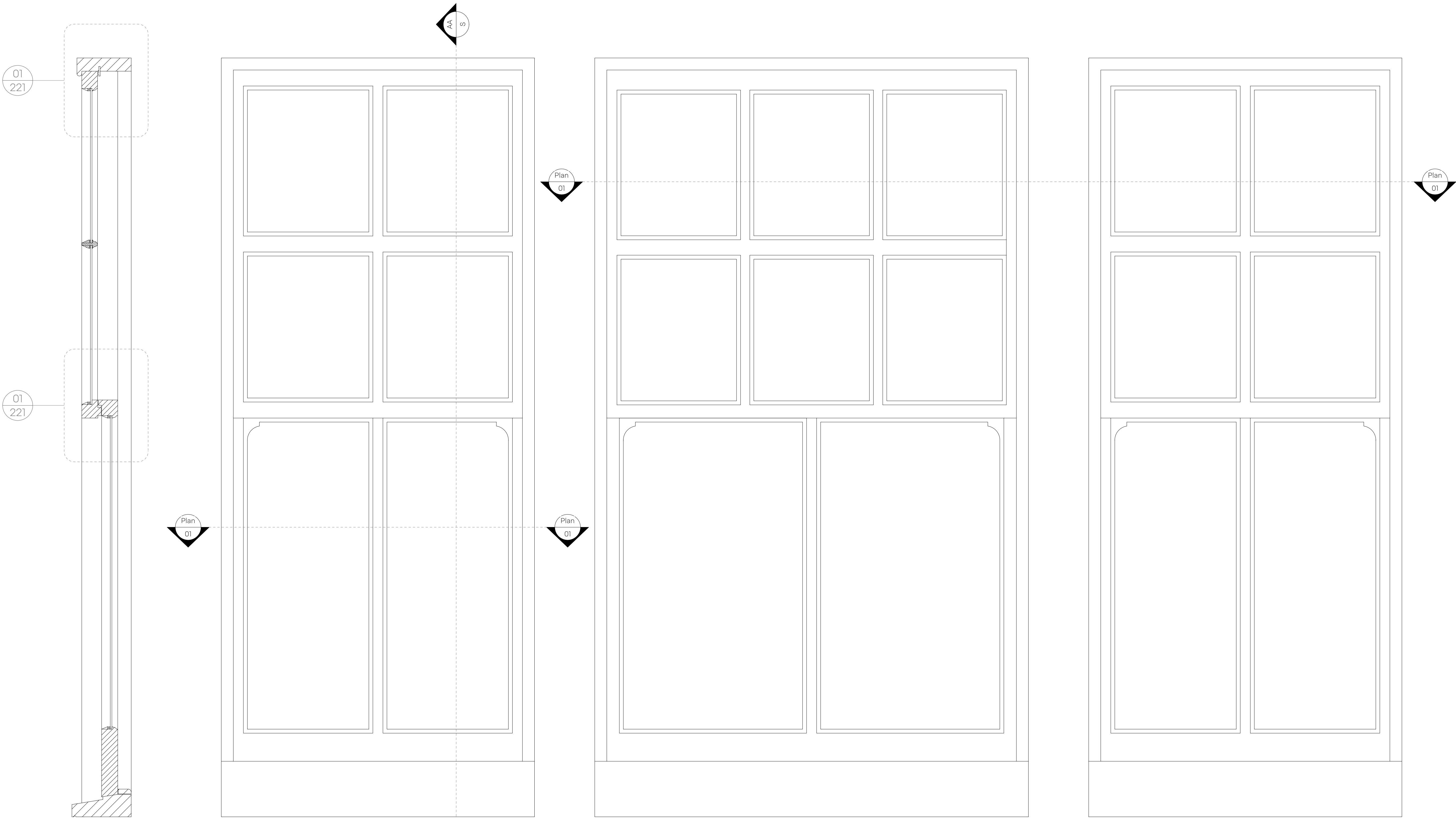
1 Existing Section AA 1:5 @A1
