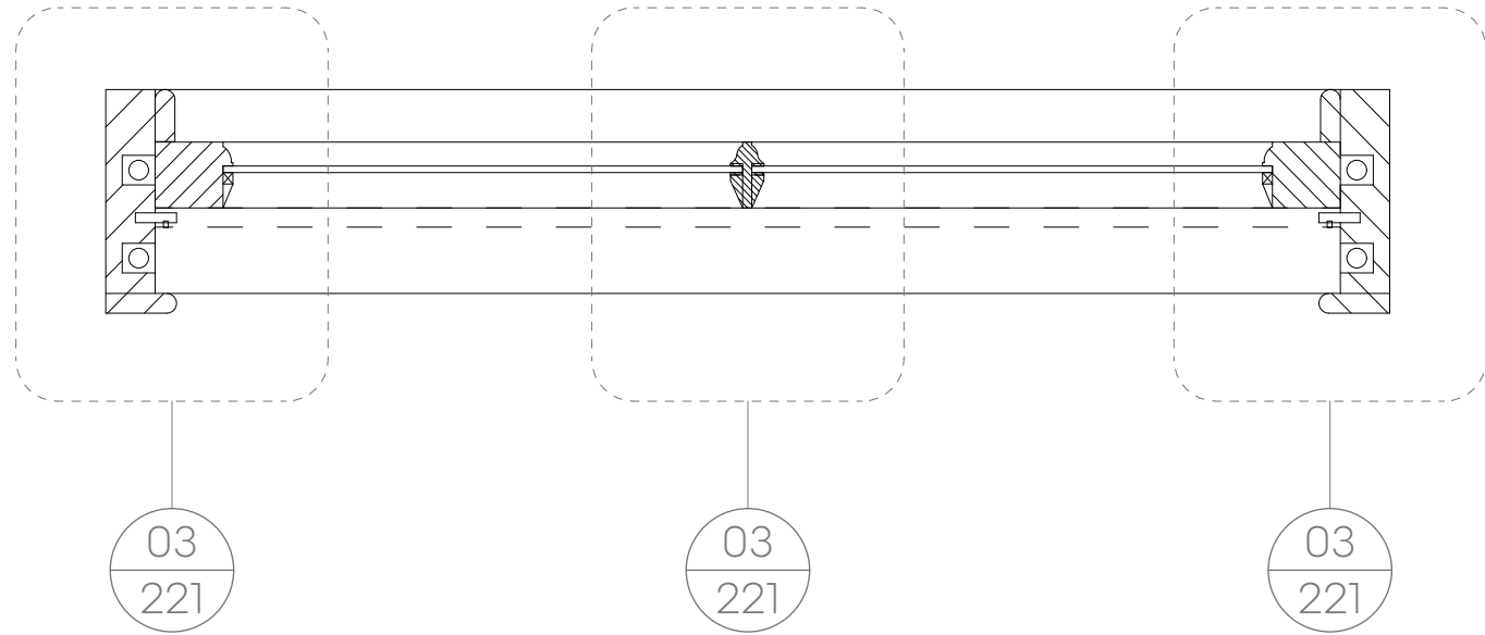
2 Existing Typical Bay Elevation 1:5 @A1
