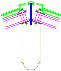
Hip Detail
