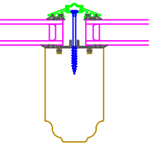
Rafter Detail
